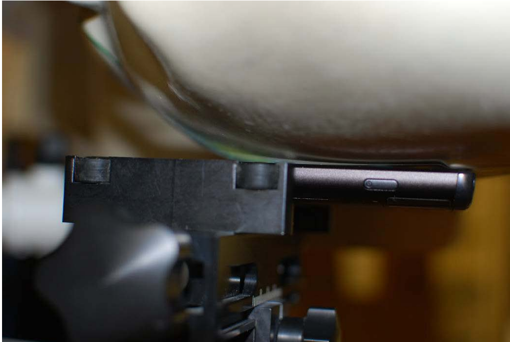
Figure 20-1 SAR Test Photo 1
