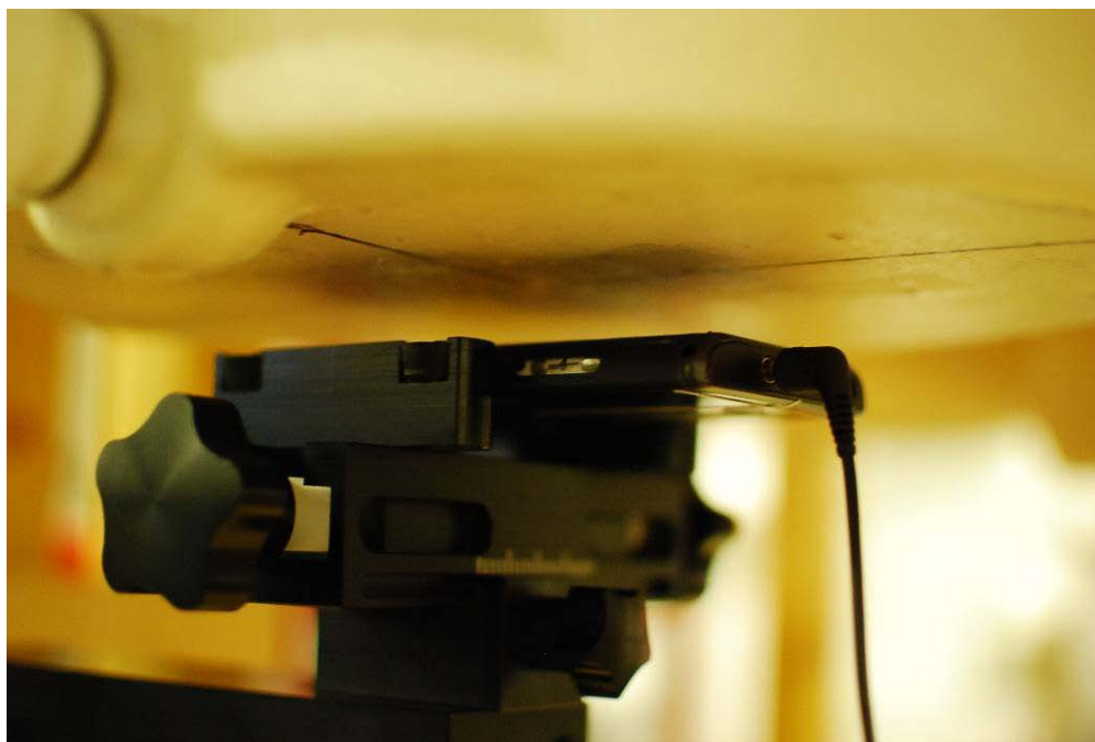
Figure 20-5 SAR Test Photo 5
