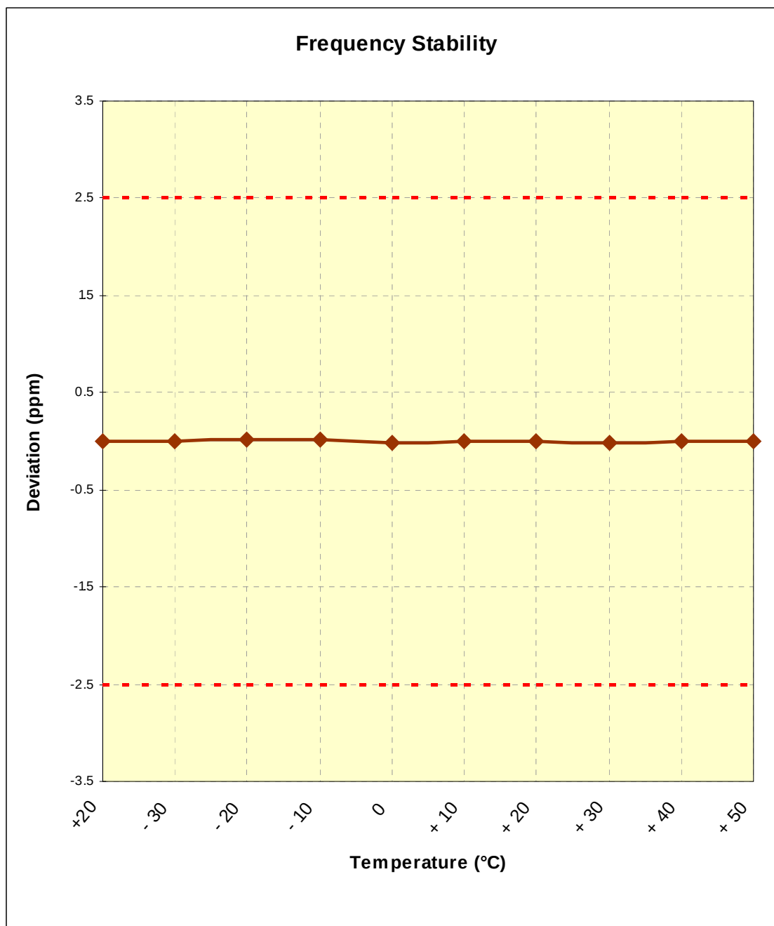
Figure 6-2. Frequency Stability Graph (20MHz BW, QPSK, Band 4 (AWS) – Ch. 20175)
