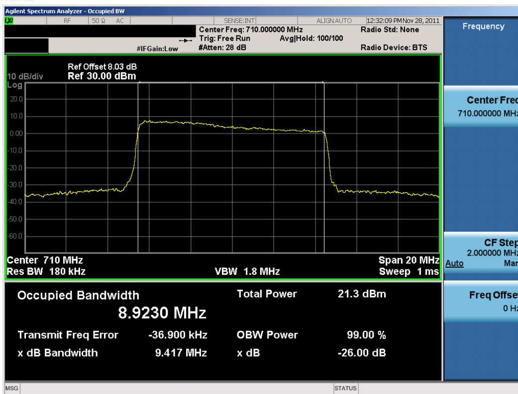
Plot 8-19. Occupied Bandwidth Plot (10MHz BW, QPSK, Band 17 – Mid Channel)
