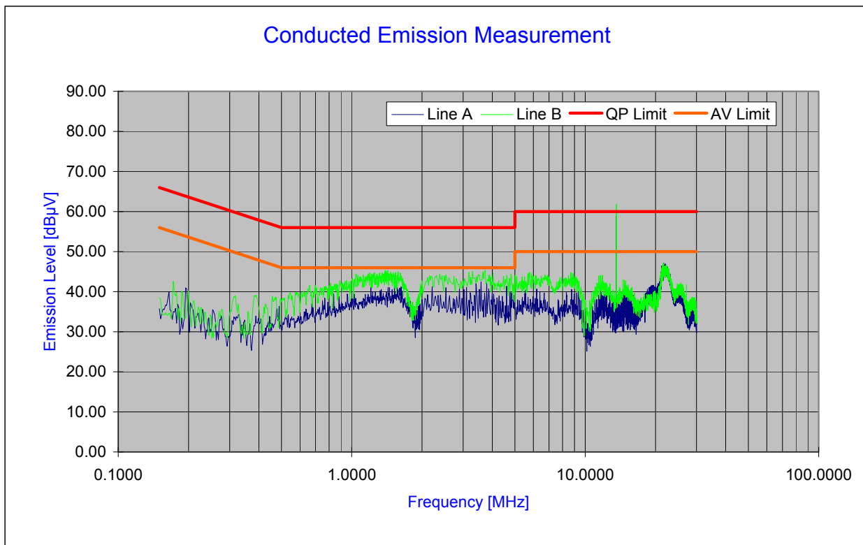
Plot 8-1. Line-Conducted Test Plot
