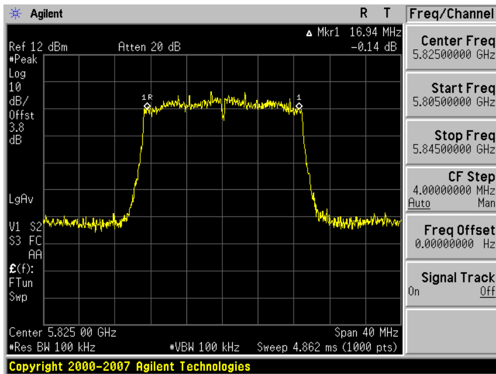
Plot 6-15. 6dB Bandwidth Plot (802.11n (5.8GHz) – Ch. 165)
