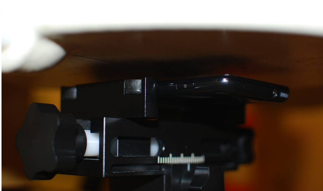
SAR Test Setup Photo 6 – Front at 1.0 cm
