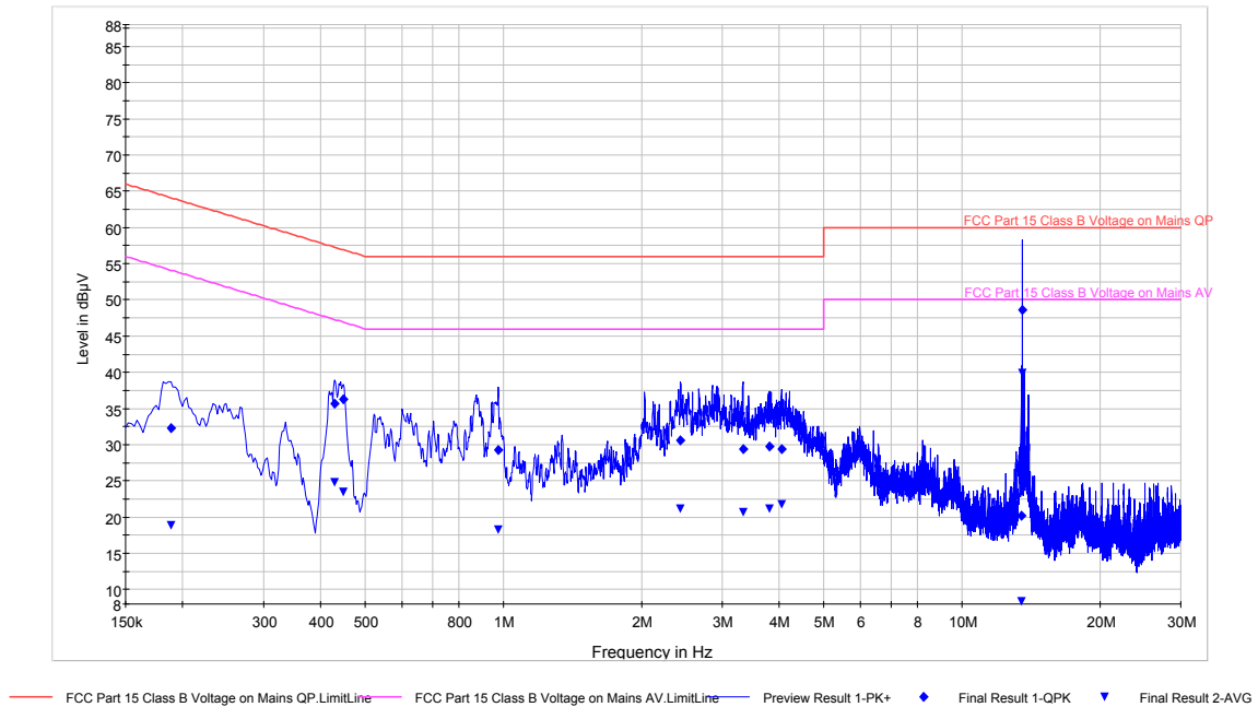
Plot 8-1. Line-Conducted Test Plot – Line 1
