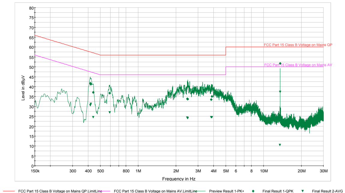
Plot 8-2. Line-Conducted Test Plot – Line N
