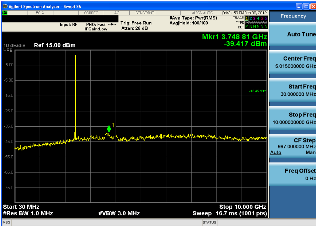
Plot 6-18. Conducted Spurious Plot (Bluetooth, 3Mbps – Ch. 39)
