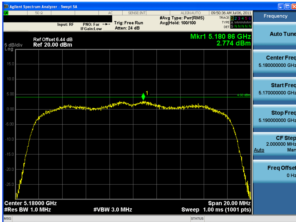
Plot 6-19. Power Spectral Density Plot (802.11a (UNII Band 1) – Ch. 36)
