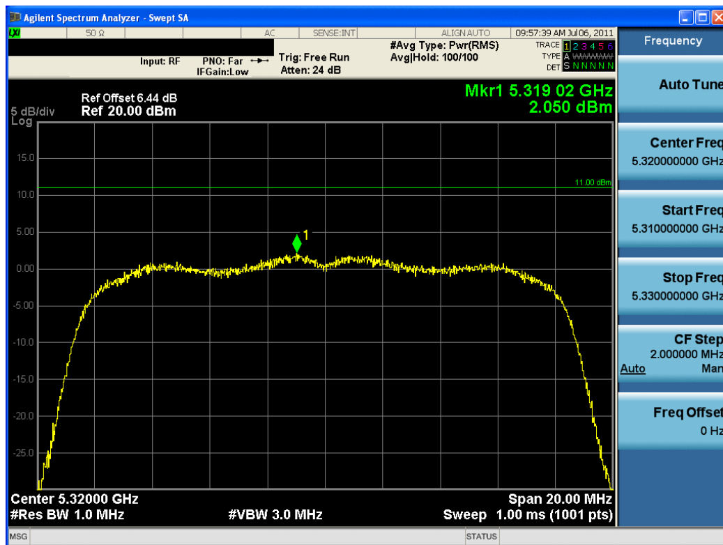
Plot 6-27. Power Spectral Density Plot (802.11a (UNII Band 2) – Ch. 64)
