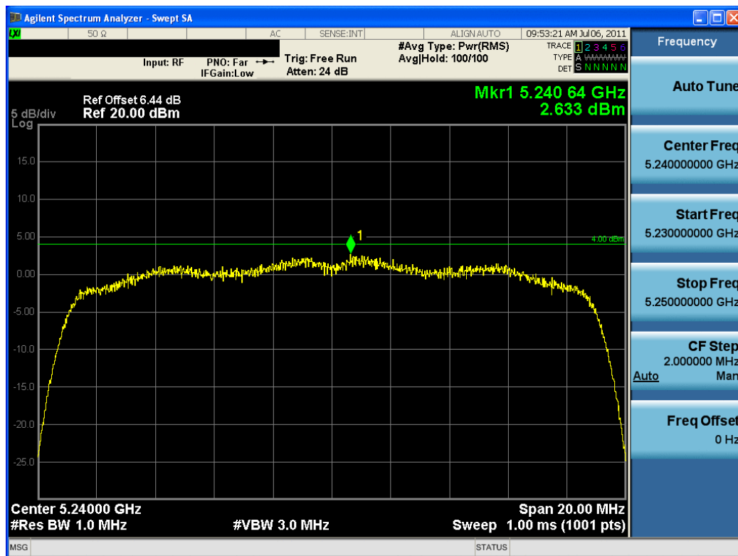
Plot 6-24. Power Spectral Density Plot (802.11n (UNII Band 1) – Ch. 48)
