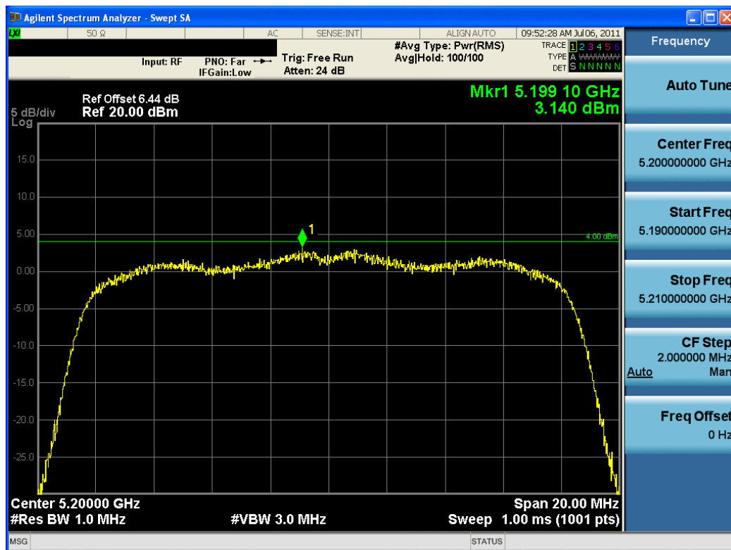
Plot 6-20. Power Spectral Density Plot (802.11a (UNII Band 1) – Ch. 40)
