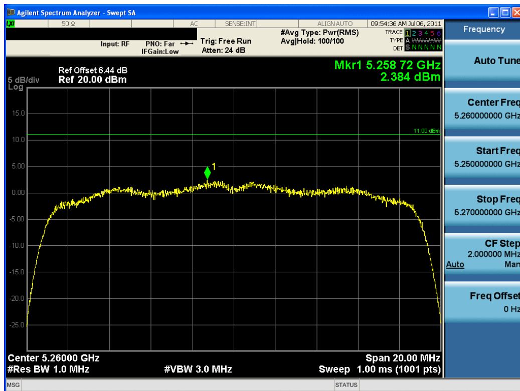
Plot 6-28. Power Spectral Density Plot (802.11n (UNII Band 2) – Ch. 52)
