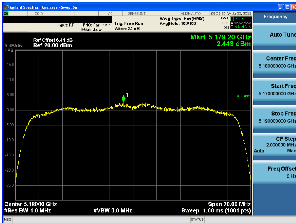
Plot 6-22. Power Spectral Density Plot (802.11n (UNII Band 1) – Ch. 36)
