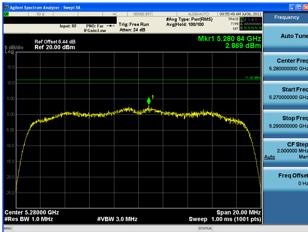
Plot 6-29. Power Spectral Density Plot (802.11n (UNII Band 2) – Ch. 56)
