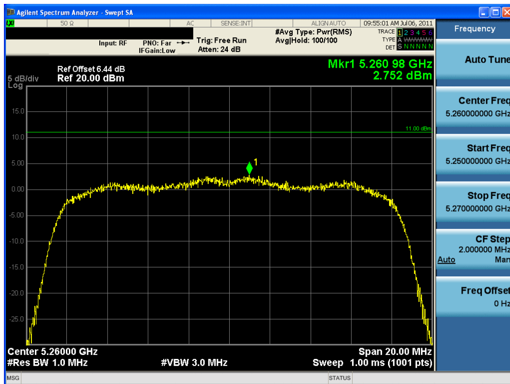
Plot 6-25. Power Spectral Density Plot (802.11a (UNII Band 2) – Ch. 52)
