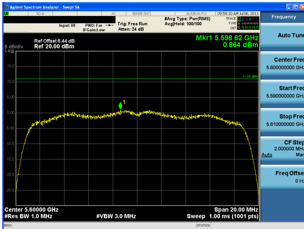
Plot 6-35. Power Spectral Density Plot (802.11n (UNII Band 3) – Ch. 120)
