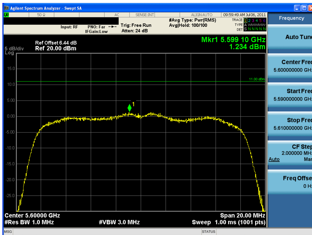
Plot 6-32. Power Spectral Density Plot (802.11a (UNII Band 3) – Ch. 120)
