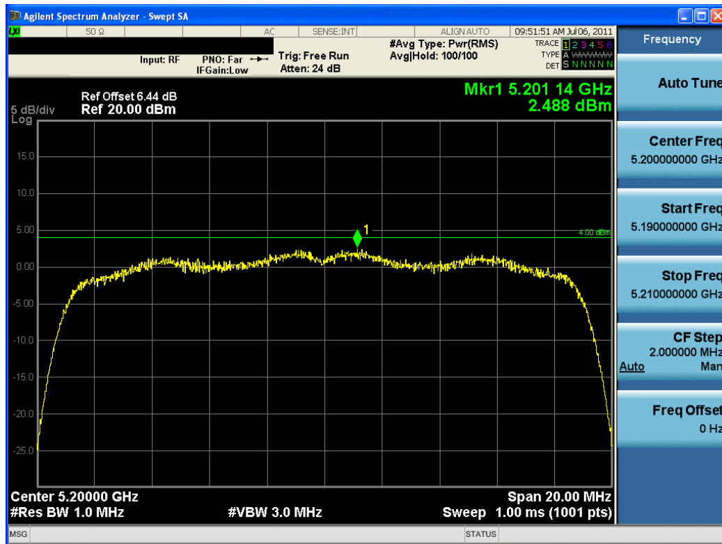
Plot 6-23. Power Spectral Density Plot (802.11n (UNII Band 1) – Ch. 40)
