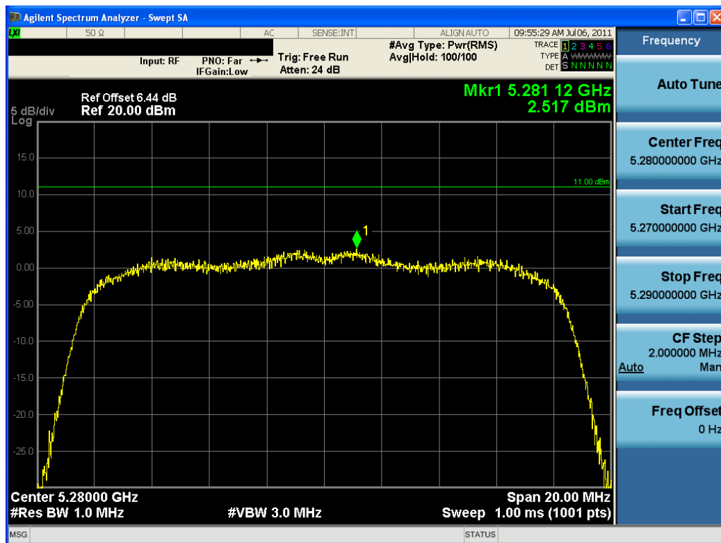
Plot 6-26. Power Spectral Density Plot (802.11a (UNII Band 2) – Ch. 56)
