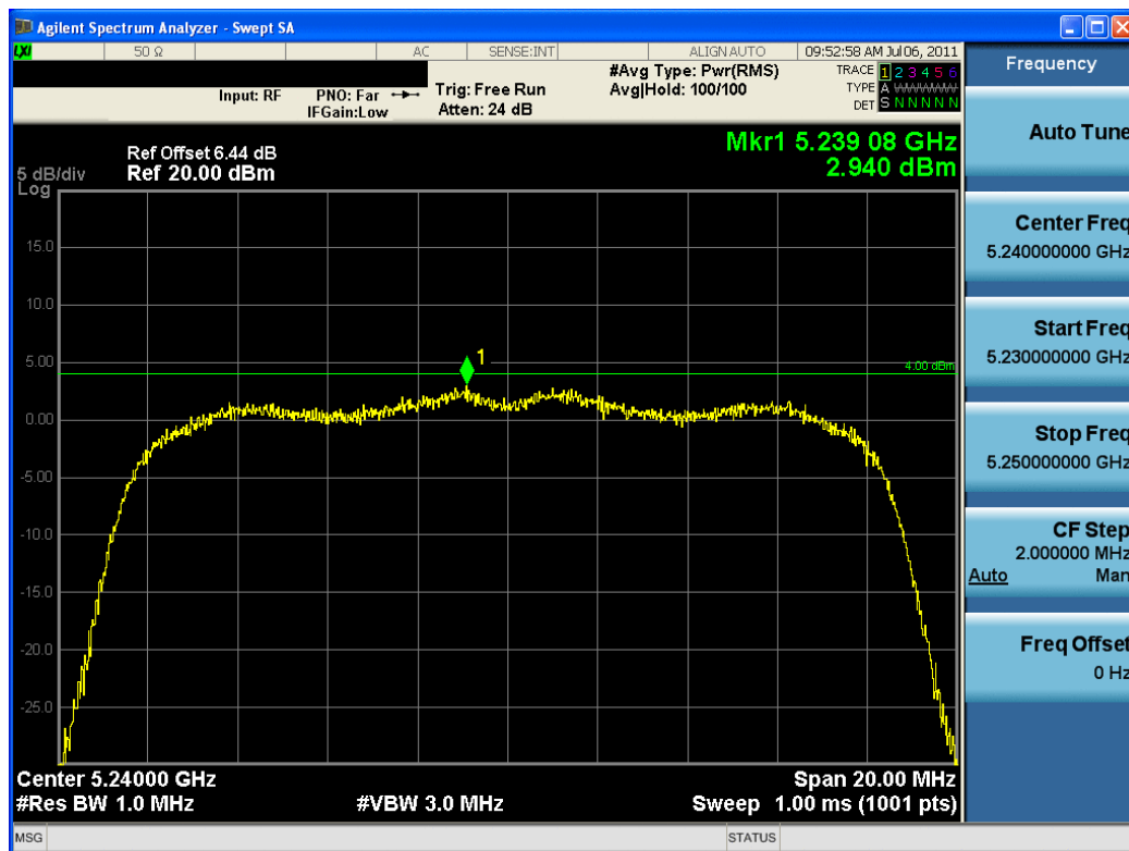
Plot 6-21. Power Spectral Density Plot (802.11a (UNII Band 1) – Ch. 48)
