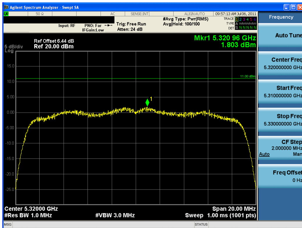
Plot 6-30. Power Spectral Density Plot (802.11n (UNII Band 2) – Ch. 64)
