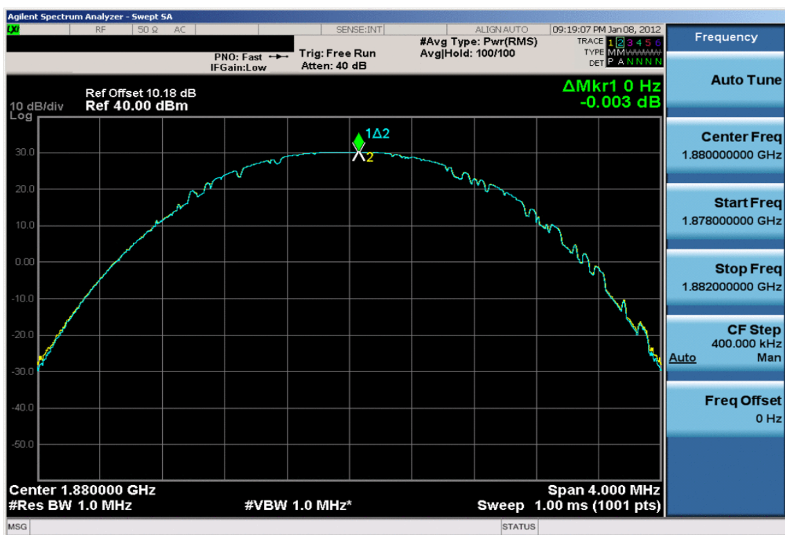
Plot 7-22. Peak-Average Ratio Plot (EDGE1900 Mode – Ch. 661)
