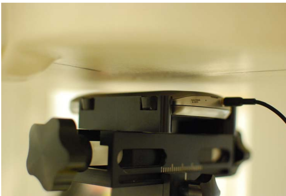
SAR Test Setup Photo 10 – Body-Worn at 1.0 cm
