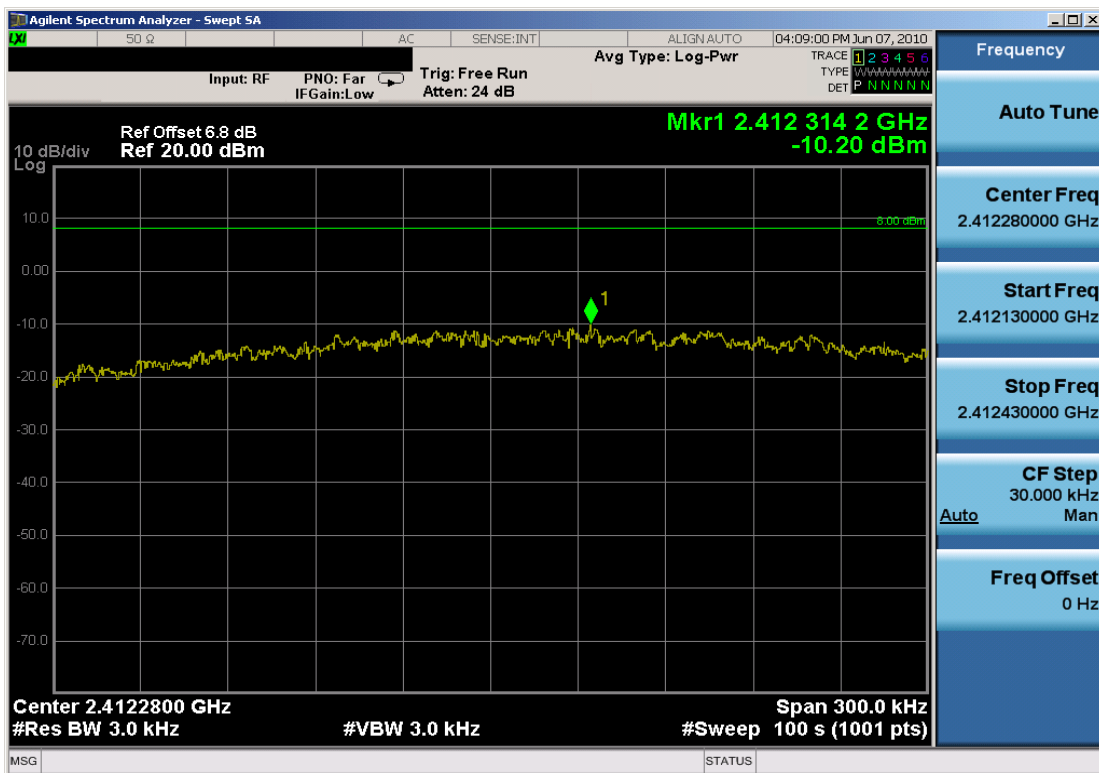
Plot 6-13. Power Spectral Density Plot (802.11g – Ch. 1)
