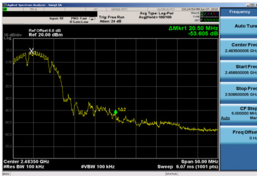
Plot 6-20. Band Edge Plot (802.11b – Ch. 11)
