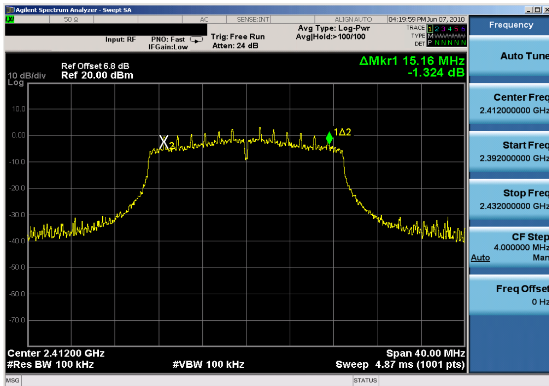
Plot 6-7. 6dB Bandwidth Plot (802.11n - Ch. 1)
