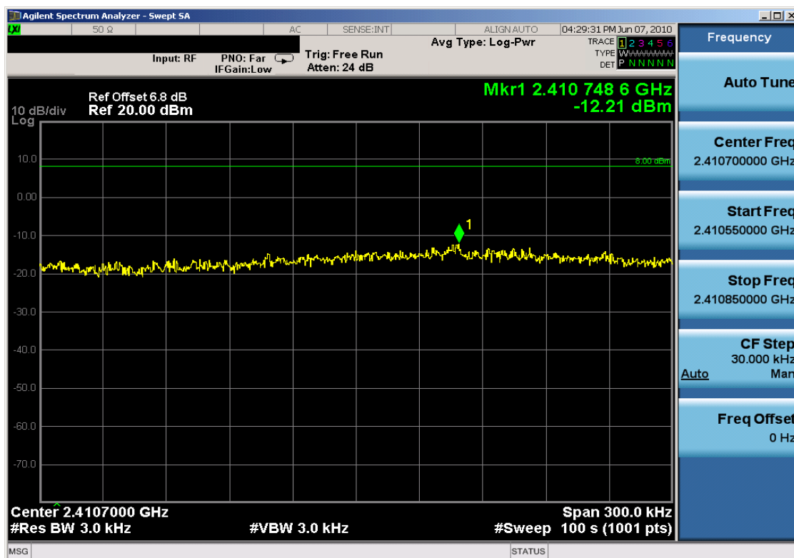
Plot 6-16. Power Spectral Density Plot (802.11n – Ch. 1)
