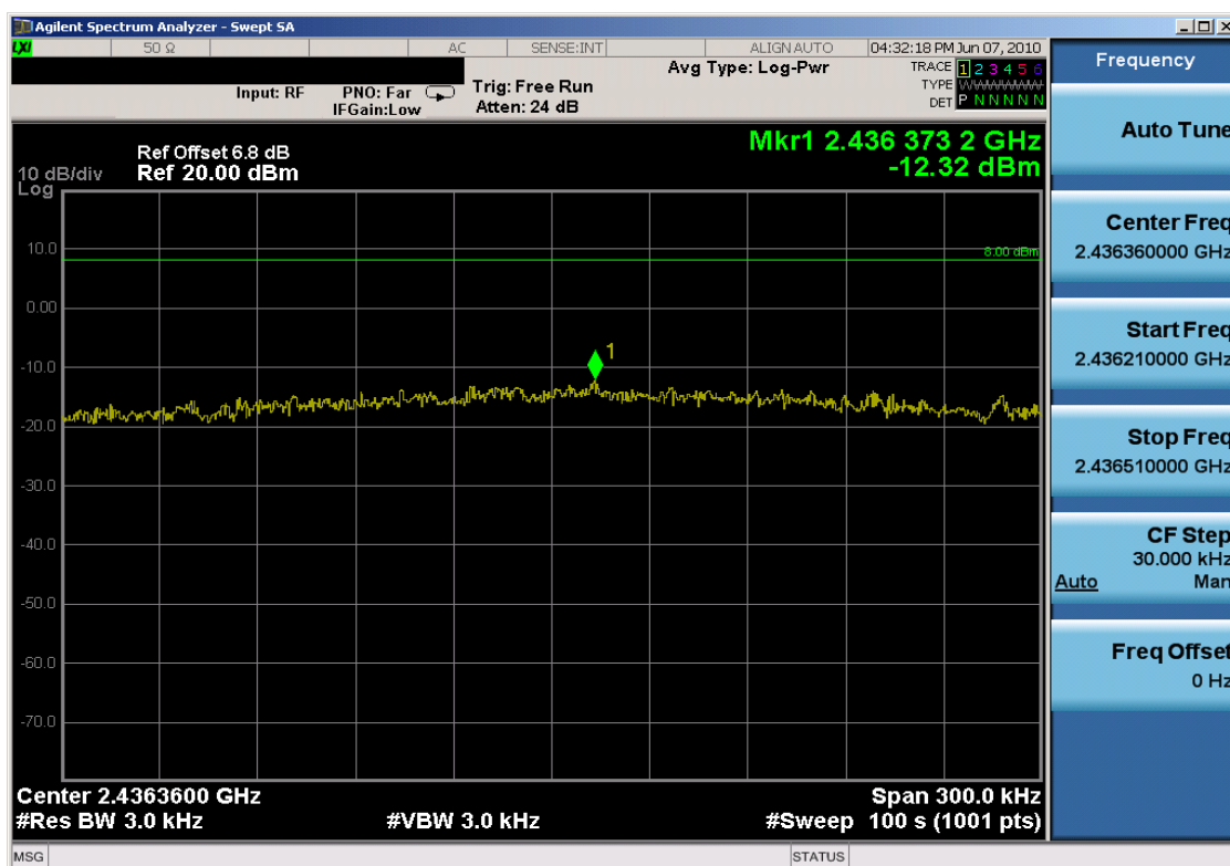
Plot 6-17. Power Spectral Density Plot (802.11n – Ch. 6)
