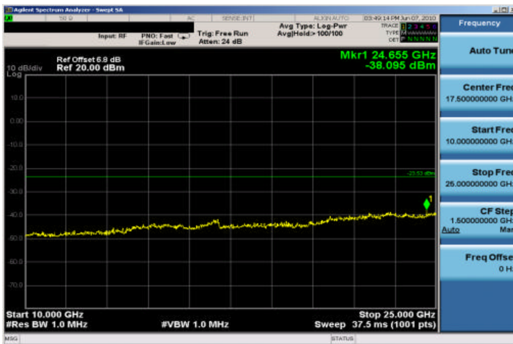
Plot 6-26. Conducted Spurious Plot (802.11b – Ch. 1)
