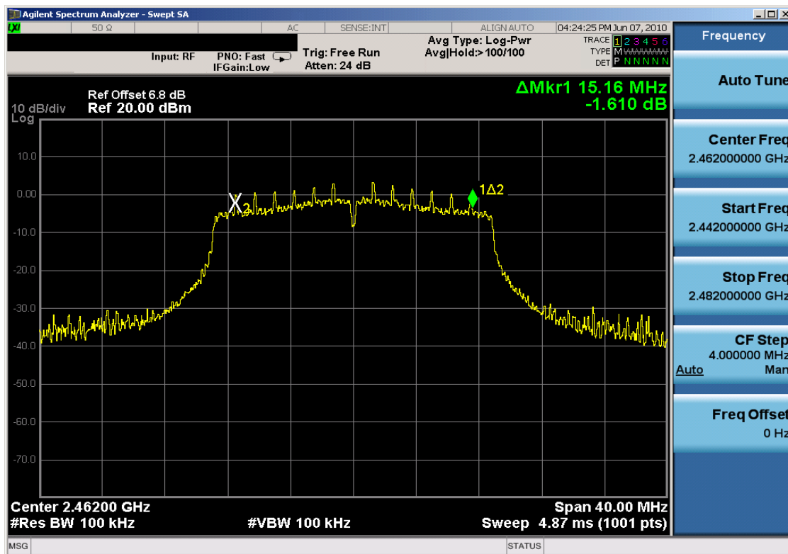
Plot 6-9. 6dB Bandwidth Plot (802.11n - Ch. 11)
