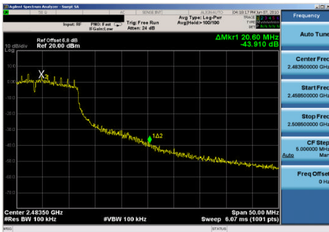
Plot 6-22. Band Edge Plot (802.11g – Ch. 11)
