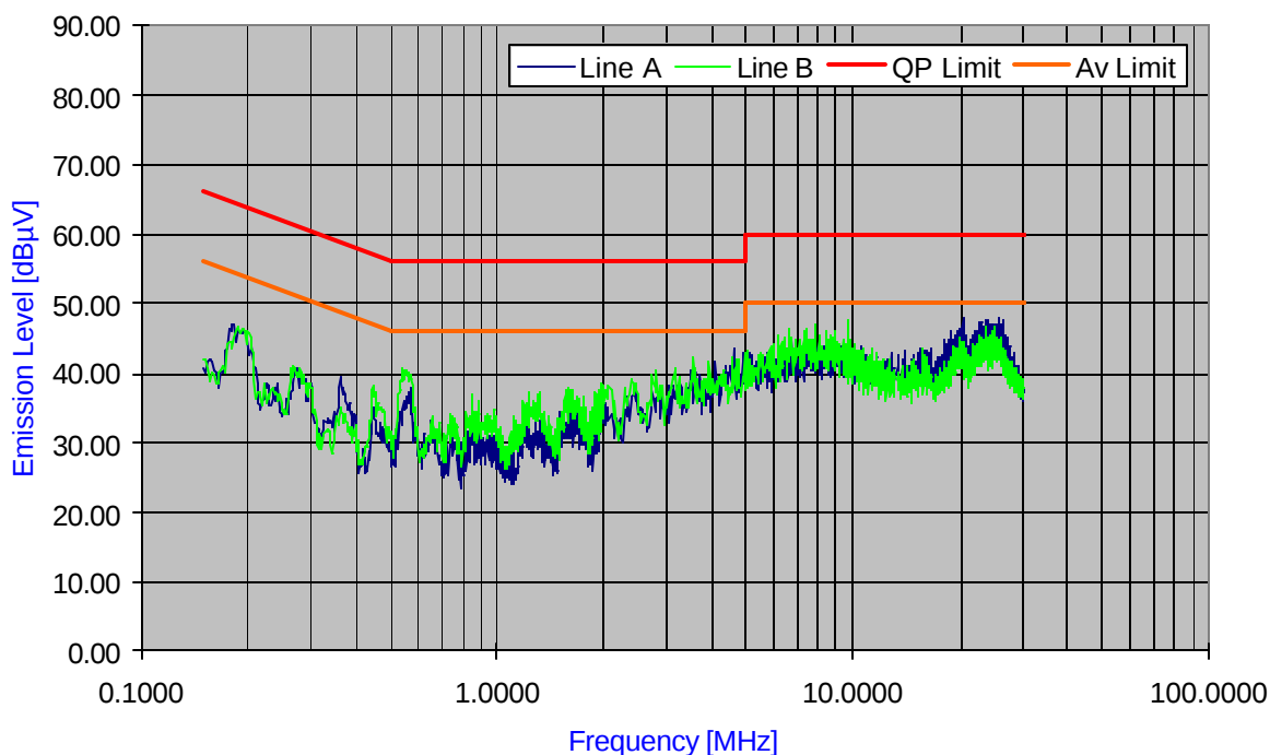
Plot 6-32. Line Conducted Plot with 802.11g
