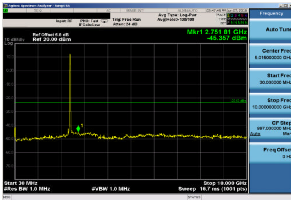
Plot 6-25. Conducted Spurious Plot (802.11b – Ch. 1)
