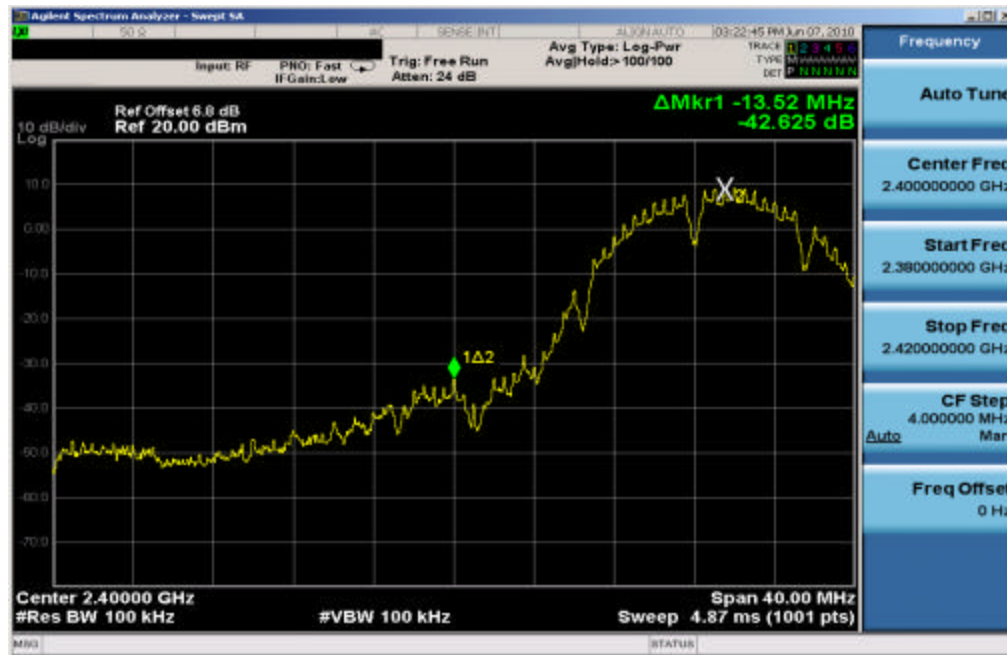
Plot 6-19. Band Edge Plot (802.11b – Ch. 1)
