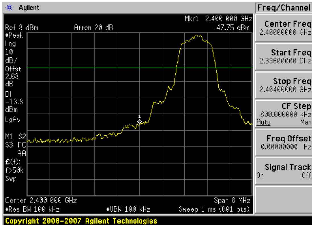
Plot 6-6. Band Edge Plot (Bluetooth 3.0 with Enhanced Data Rates – Ch. 0)
