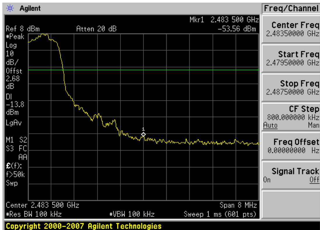
Plot 6-7. Band Edge Plot (Bluetooth 3.0 with Enhanced Data Rates – Ch. 78)
