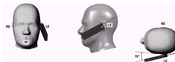
Figure 9-2 Front, Side and Top View of Ear/15° Tilt Position
