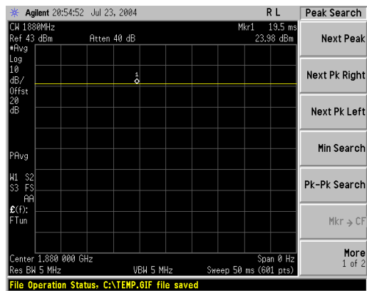
Figure 8.10 WCDMA1900 CW Signal
