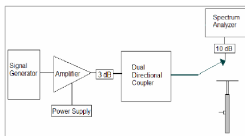
Figure 8.2 Setup to Peak Power using Spectrum Analyzer
