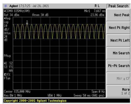
Figure 8. WCDMA850 80% AM Signal
