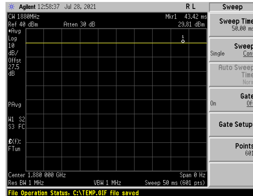
Figure 8.4 GSM1900 CW Signal
