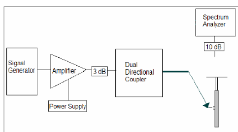
Figure 8.1 Setup to Dipole
