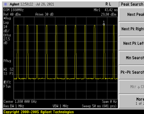
Figure 8.3 GSM1900 Signal
