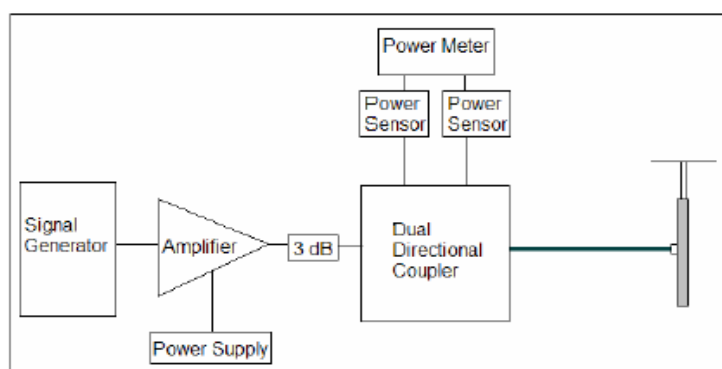
Figure 7.1 Dipole Validation Test Setup
