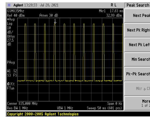
Figure 8.6 GSM850 Signal
