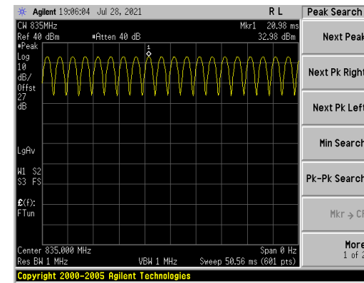
Figure 8.8 GSM850 80% AM Signal
