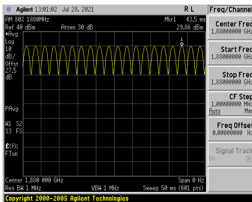
Figure 8.5 GSM1900 80% AM Signal
