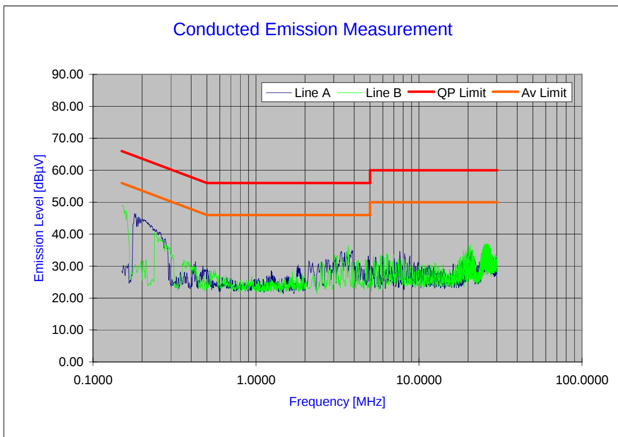
Plot 6-20. Line Conducted Plot with 802.11g
