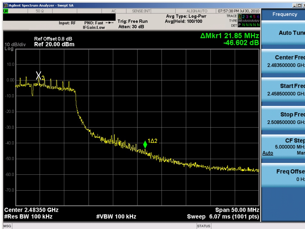
Plot 6-12. Band Edge Plot (802.11n – Ch. 11)
