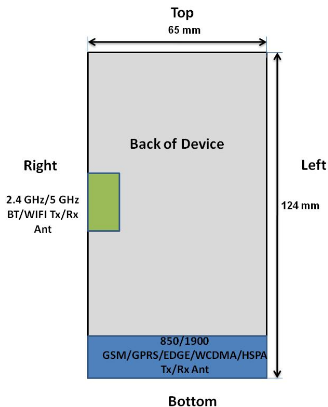
Figure 13-1 Identification of Sides for SAR Testing (Front View)
