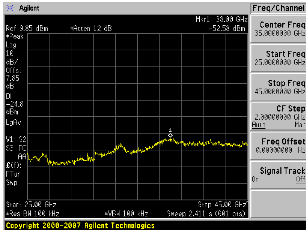
Plot 6-49. Conducted Spurious Plot (802.11a – Ch. 149)
