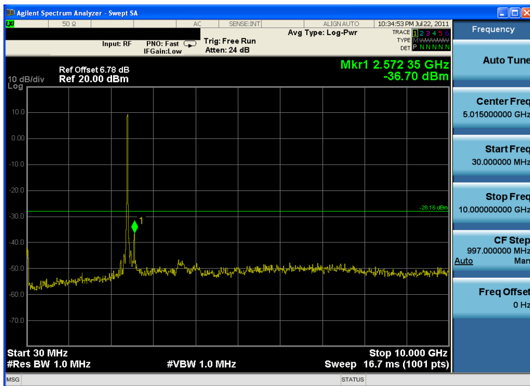
Plot 6-41. Conducted Spurious Plot (802.11b – Ch. 1)
