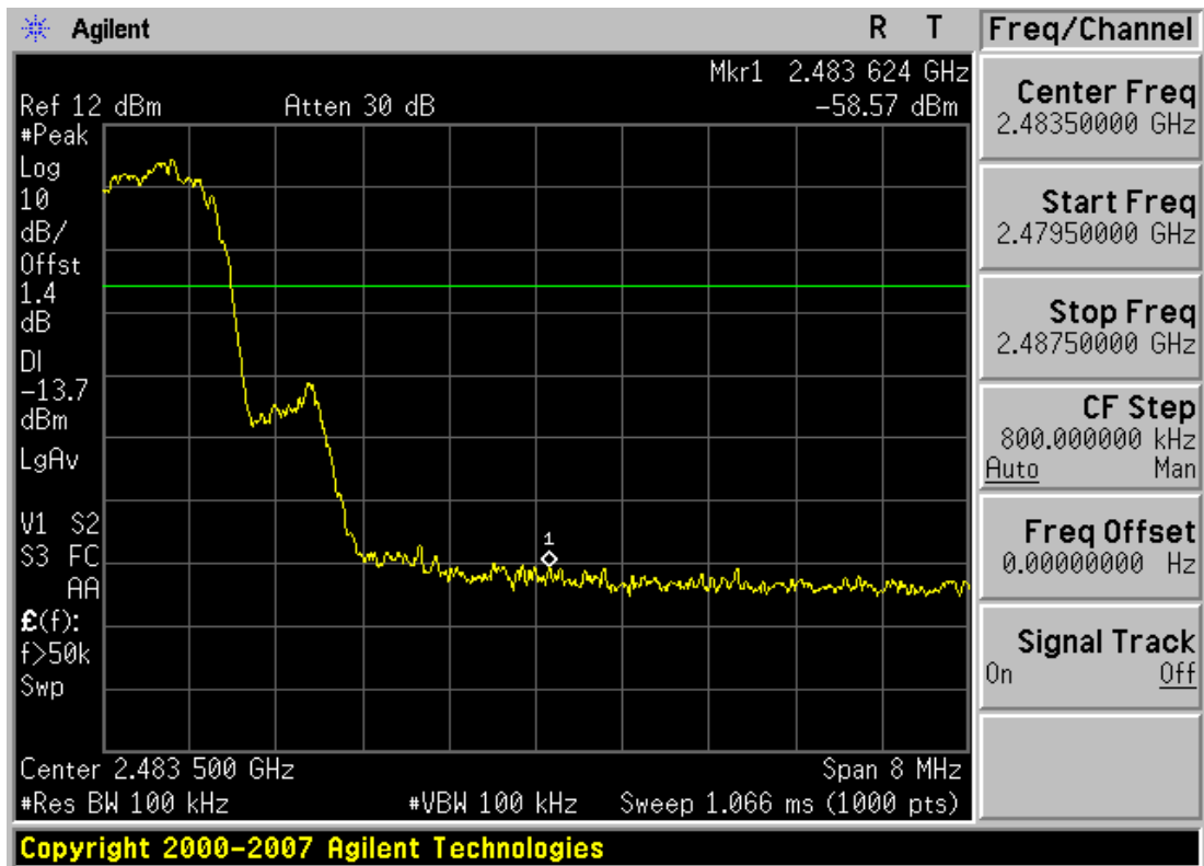
Plot 6-13. Band Edge Plot (Bluetooth, 3Mbps – Ch. 78)
