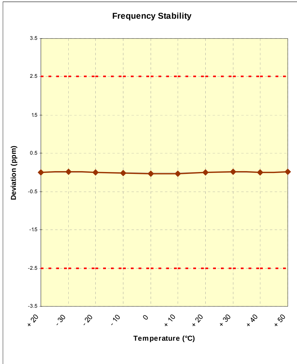
Figure 6-1. Frequency Stability Graph (Cellular GSM Mode – Ch. 190)
