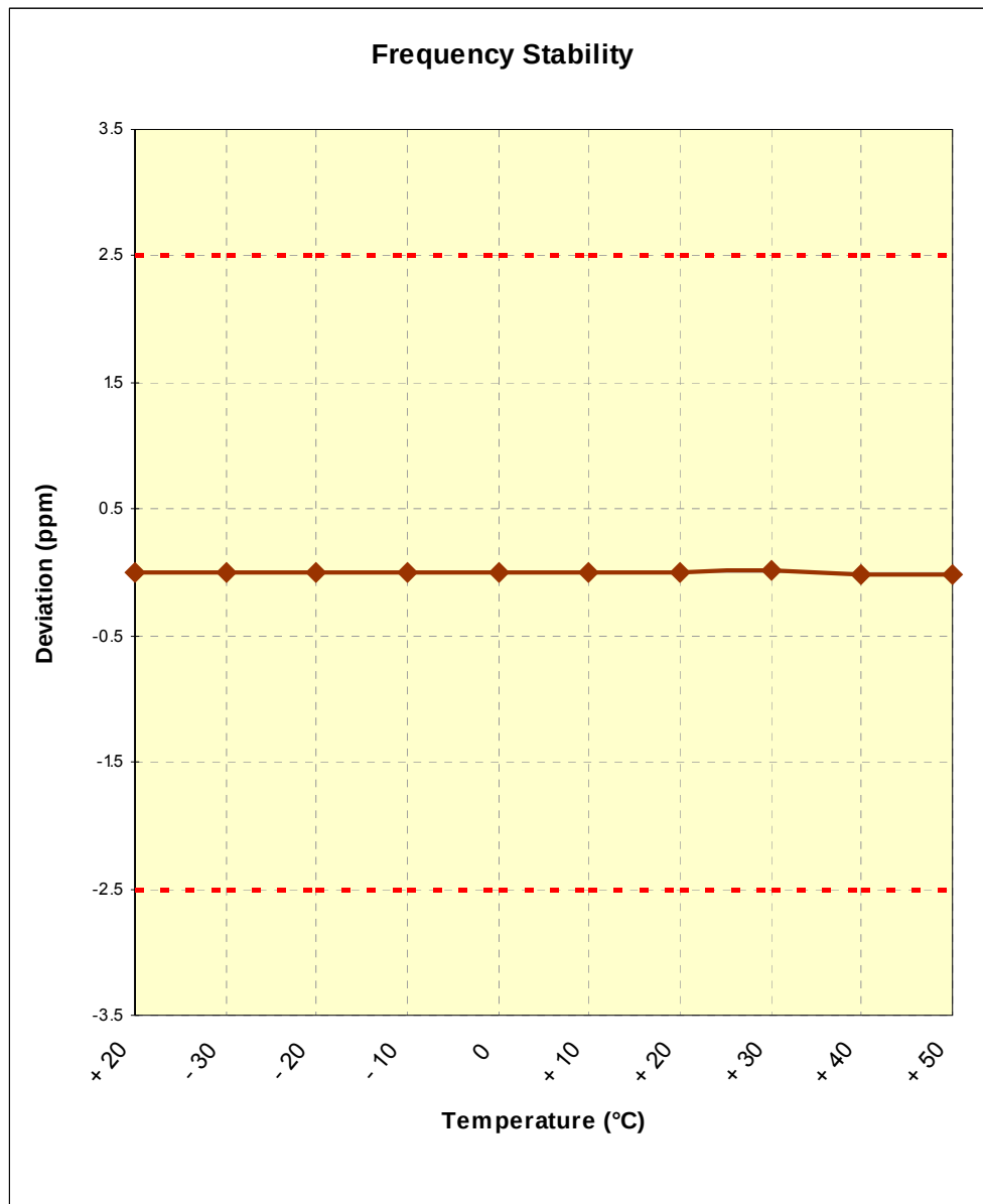
Figure 6-3. Frequency Stability Graph (PCS GSM Mode – Ch. 661)
