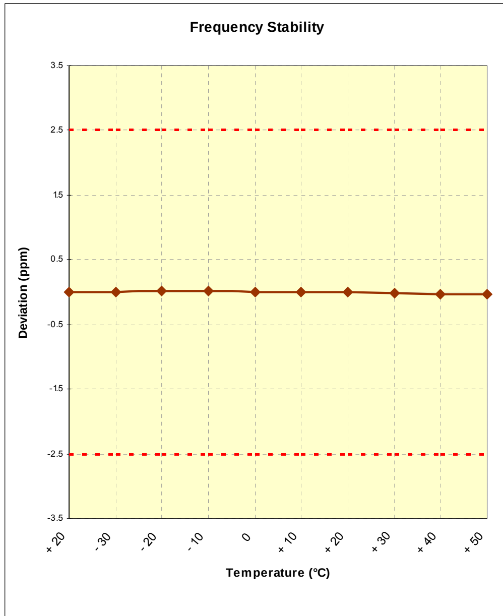
Figure 6-2. Frequency Stability Graph (Cellular WCDMA Mode – Ch. 4183)
