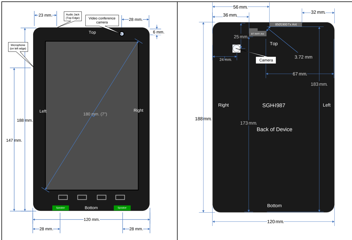
Figure 11-1 Antenna & Key Feature Diagram
