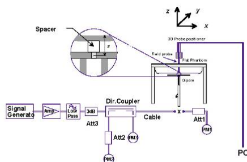
Figure 10-1 System Verification Setup Diagram
