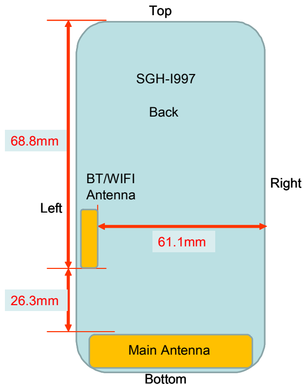
Figure 13-1 Identification of Sides for SAR Testing
