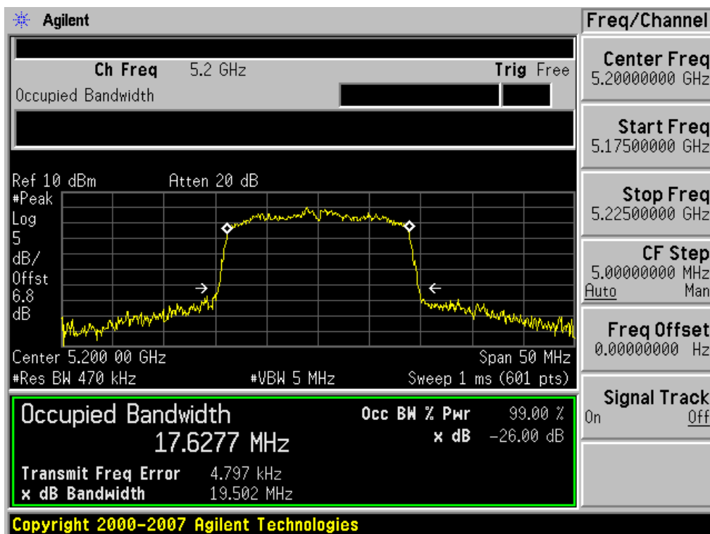
Plot 6-5. 26dB Bandwidth Plot (802.11n (UNII) – Ch. 40)
