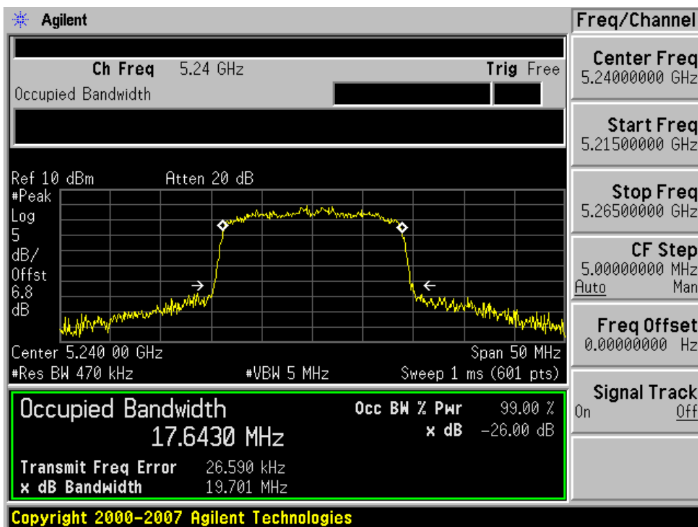
Plot 6-6. 26dB Bandwidth Plot (802.11n (UNII) – Ch. 48)
