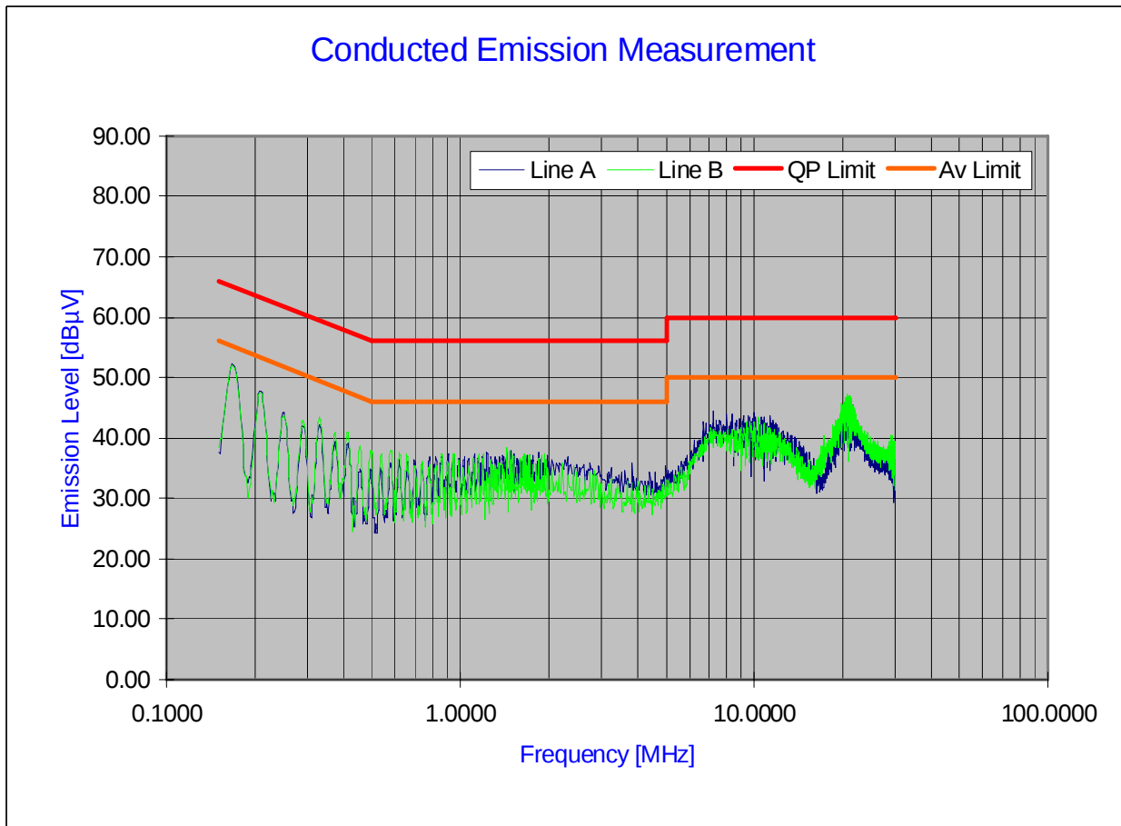
Plot 6-54. Line Conducted Plot with 802.11n
