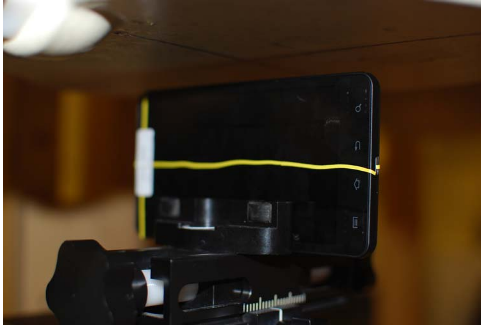
Figure 21-7 SAR Test Setup Photo 7 – Right at 1.0 cm
