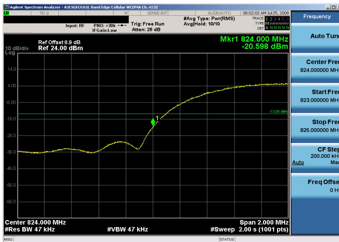
Plot 7-24. Band Edge Plot (Cellular WCDMA Mode – Ch. 4132)
