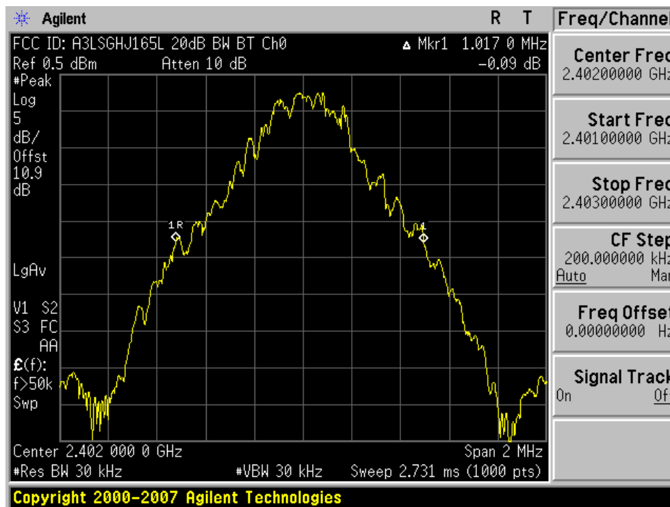
Plot 6-1. 20dB Bandwidth Plot (Bluetooth 2.0 – Ch. 0)
