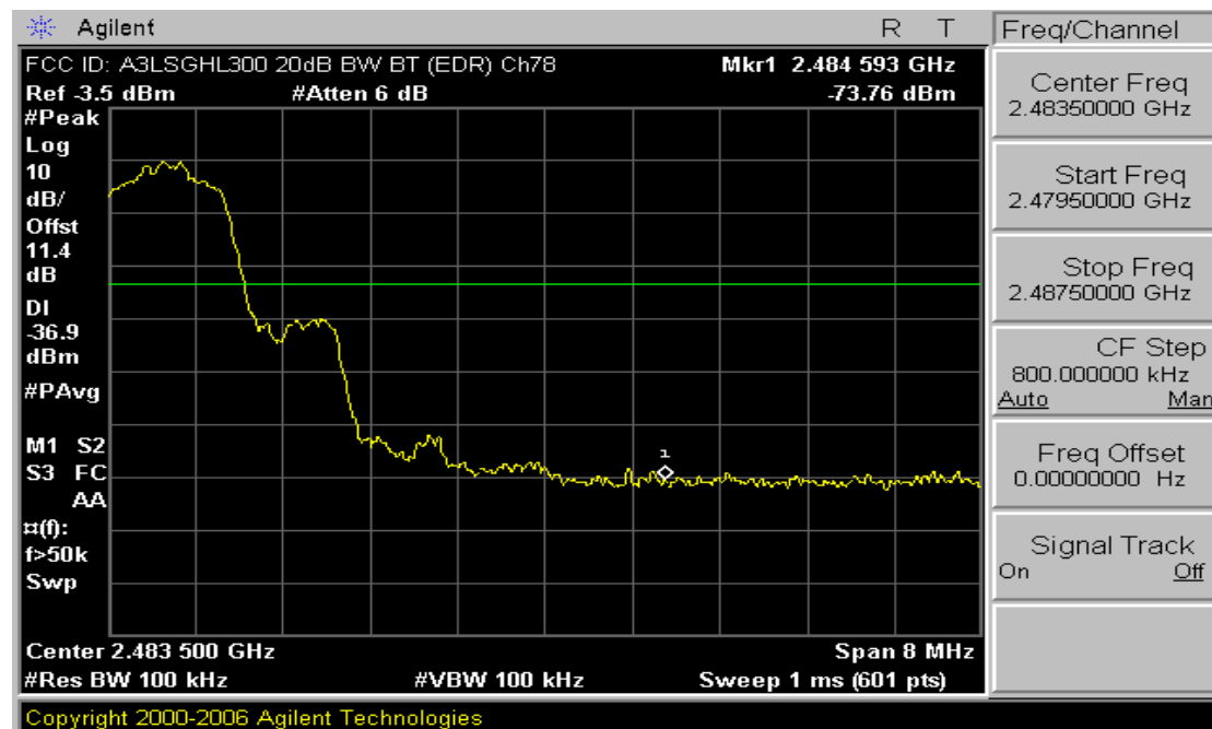
Plot 6-5. Band Edge Plot (Bluetooth 2.0 with Enhanced Data Rate – Ch. 78)
