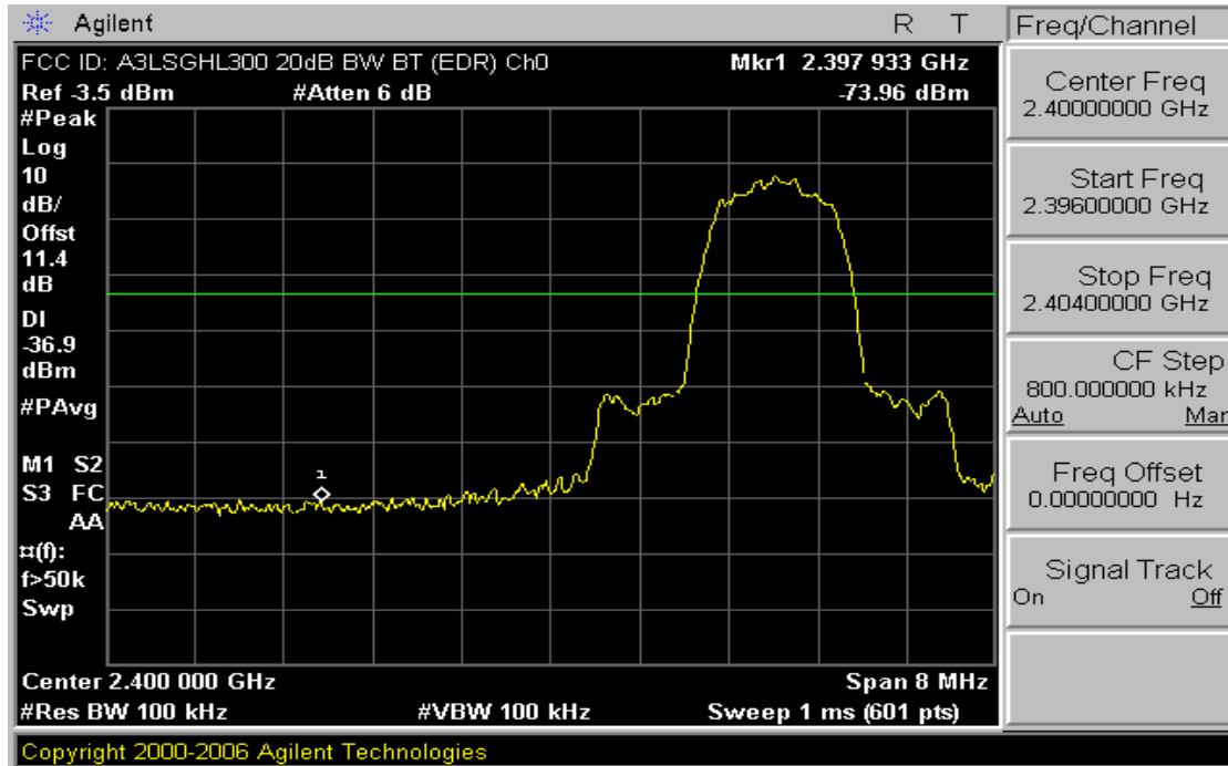
Plot 6-4. Band Edge Plot (Bluetooth 2.0 with Enhanced Data Rate – Ch. 0)
