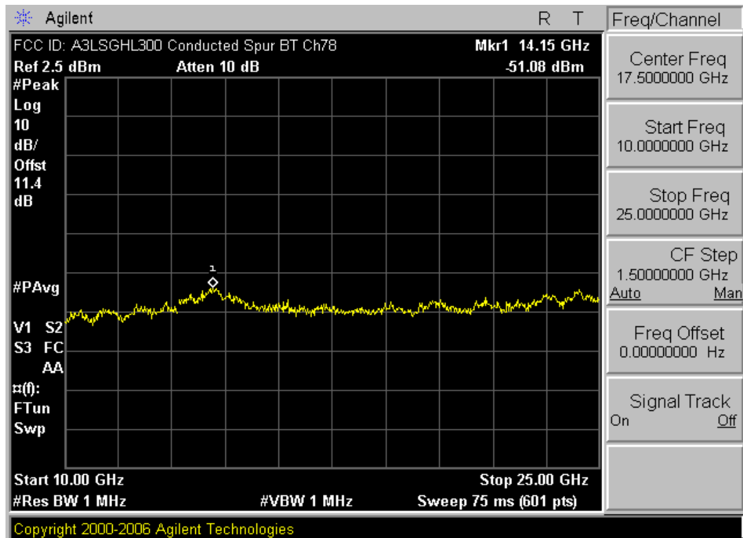
Plot 6-15. Conducted Spurious Plot (Bluetooth – Ch. 78)
