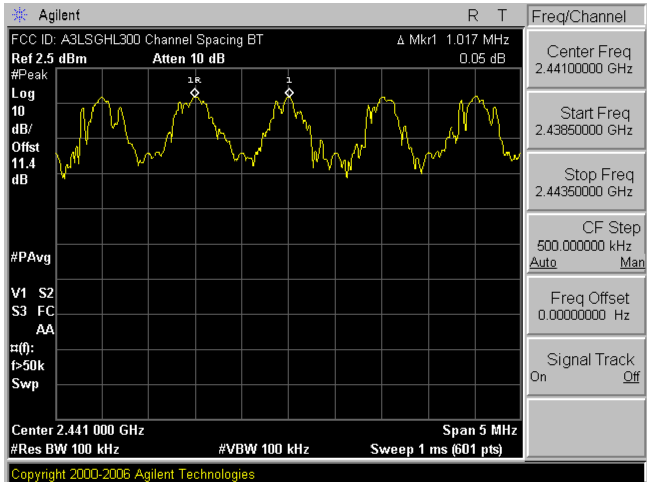
Plot 6-6. Channel Spacing Plot (Bluetooth)
