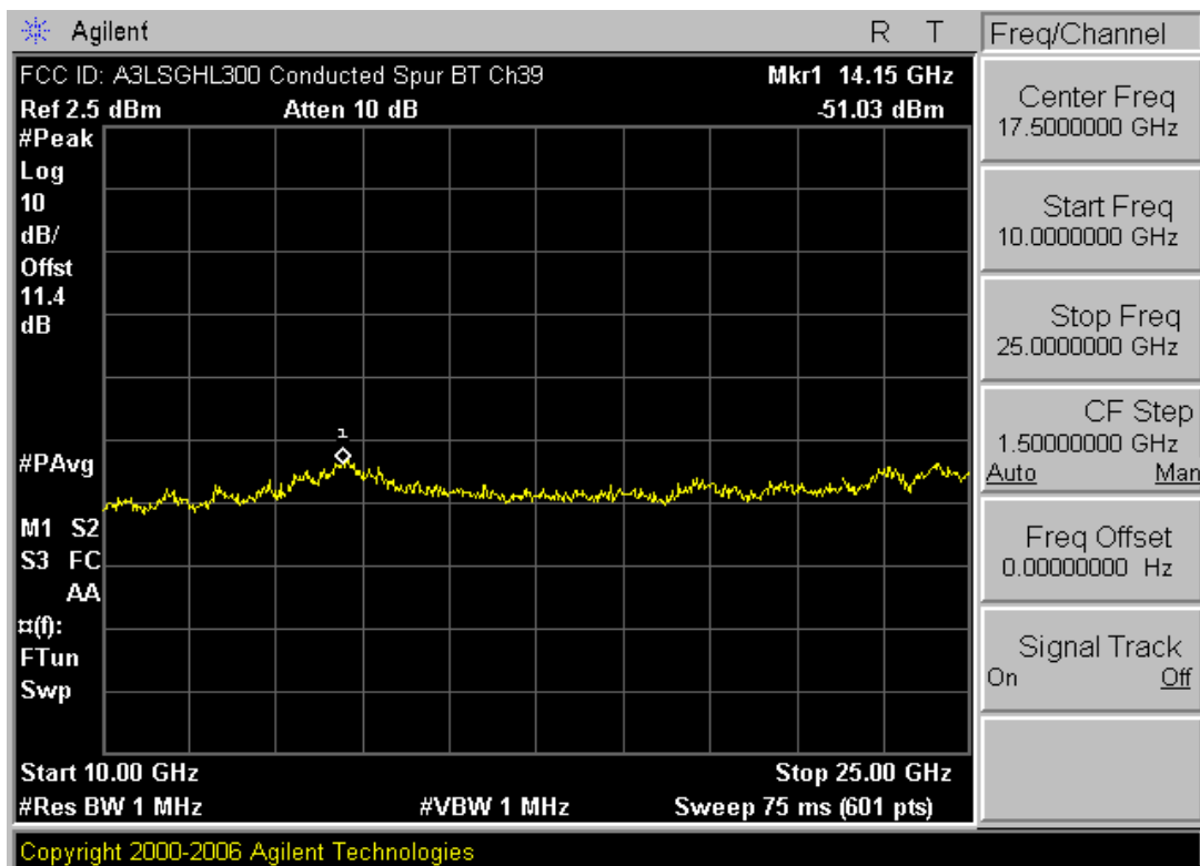
Plot 6-13. Conducted Spurious Plot (Bluetooth – Ch. 39)
