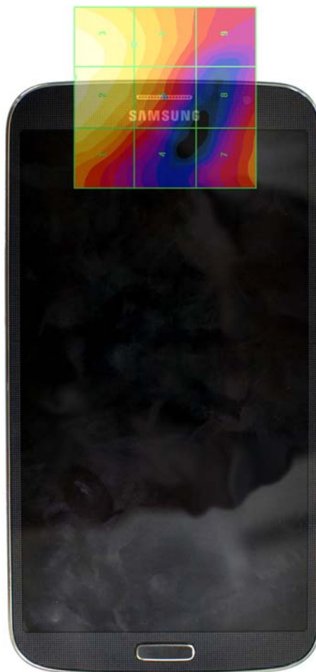
Figure 18-4 E-Field WD Scan overlay
