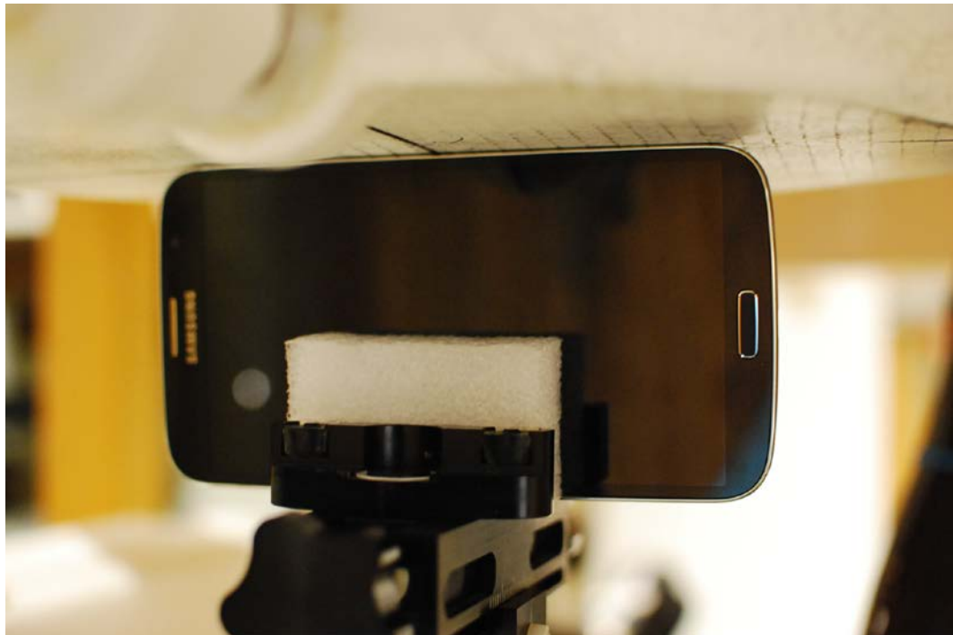
SAR Test Setup Photo 14: Right at 0.0 cm
