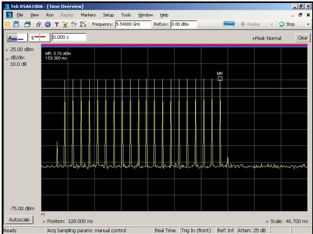
Figure 6-1. Type 1 Radar Pulse
