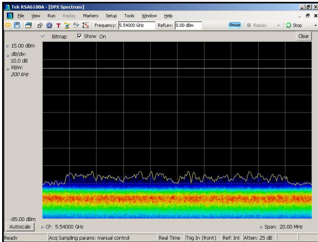
Figure 6-2. Real-Time Spectrum Display, No WLAN Traffic
