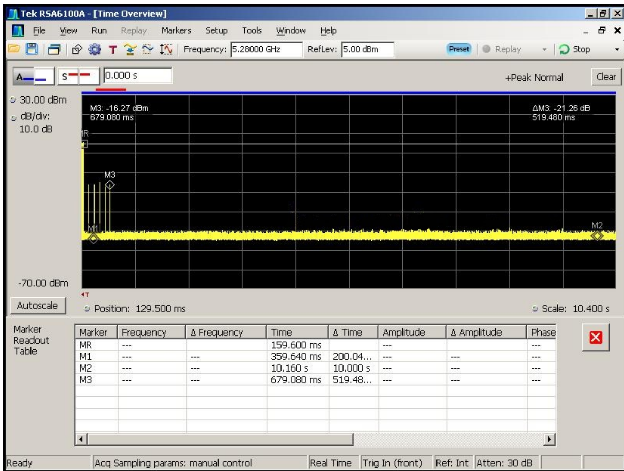
Figure 5-4. Channel Move Time (< 10sec)
