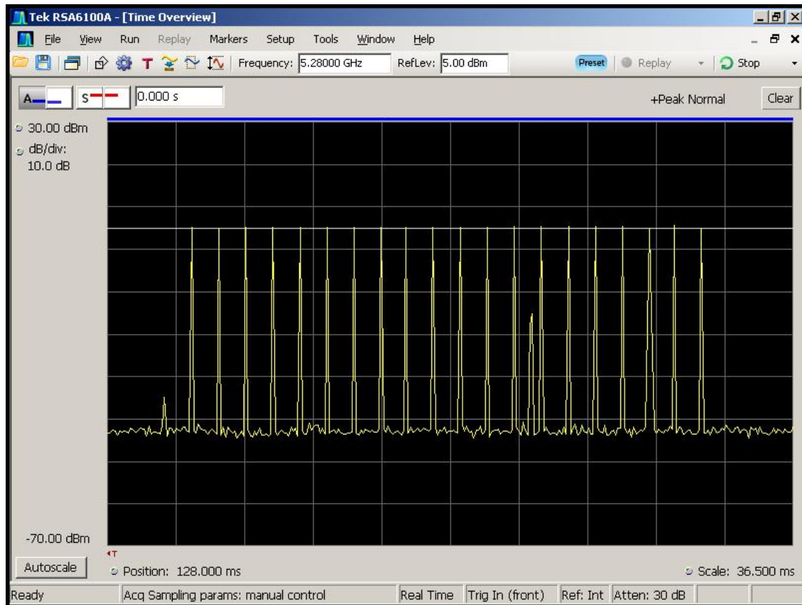
Figure 5-1. Type 1 Radar Pulse
