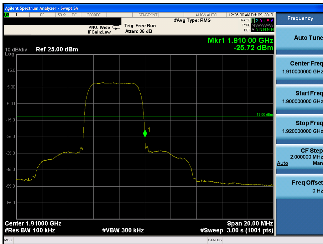
Plot 7-57. Band Edge Plot (PCS WCDMA Mode – Ch. 9538)
