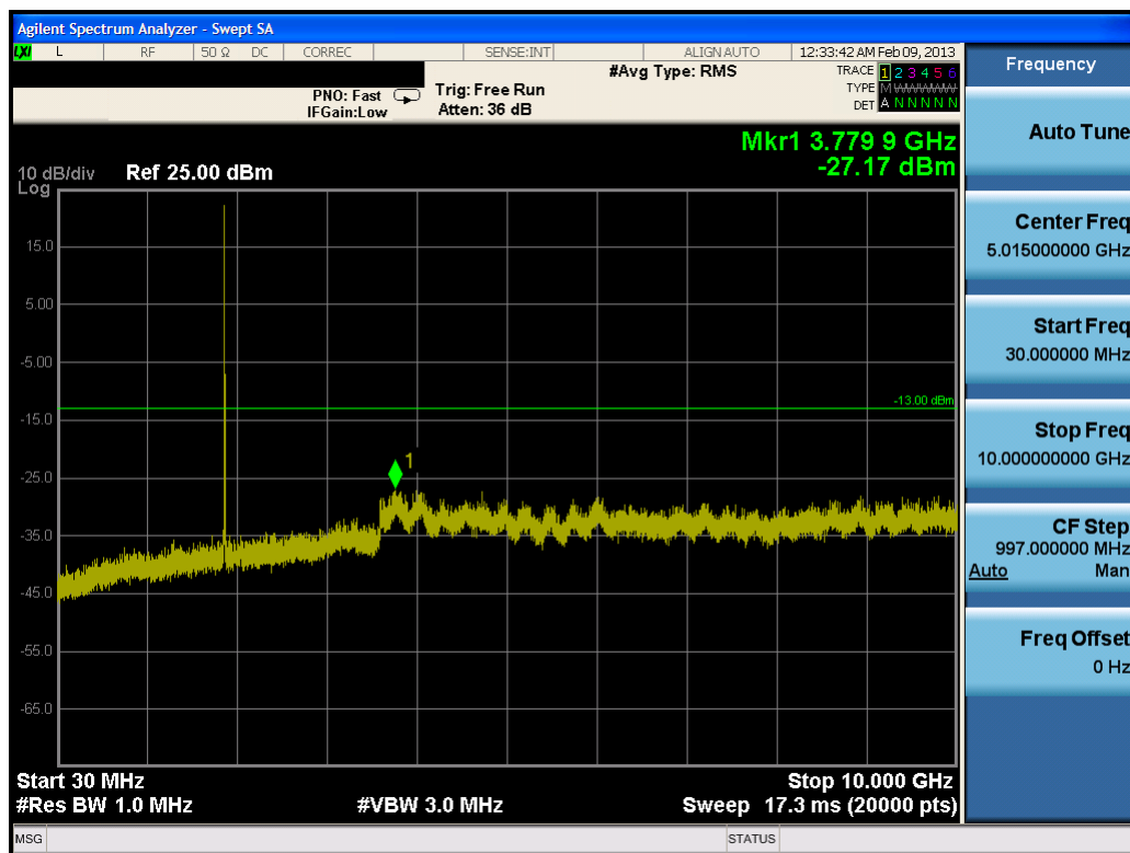
Plot 7-51. Conducted Spurious Plot (PCS WCDMA Mode – Ch. 9400)
