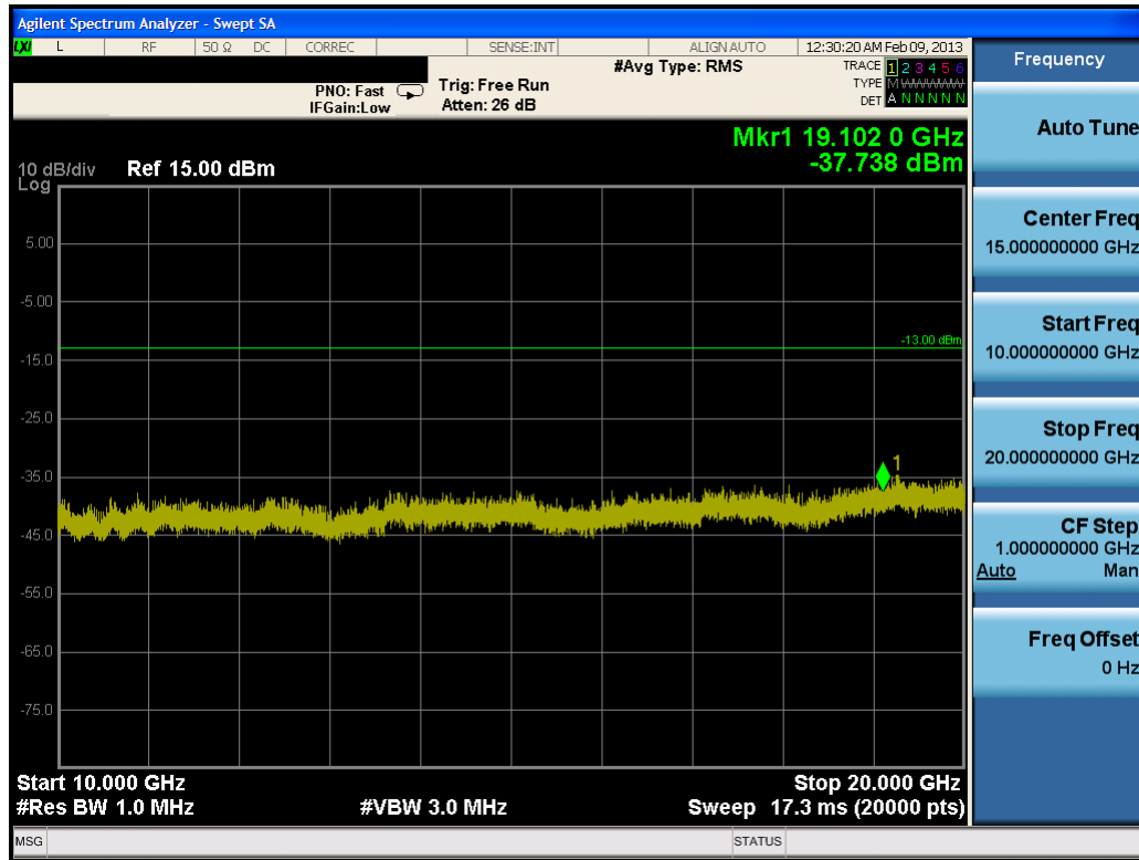
Plot 7-48. Conducted Spurious Plot (PCS WCDMA Mode – Ch. 9262)
