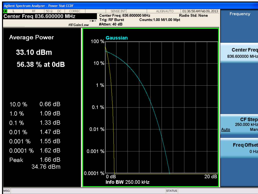
Plot 7-7. Peak-Average Ratio Plot (Cellular GSM Mode – Ch. 190)
