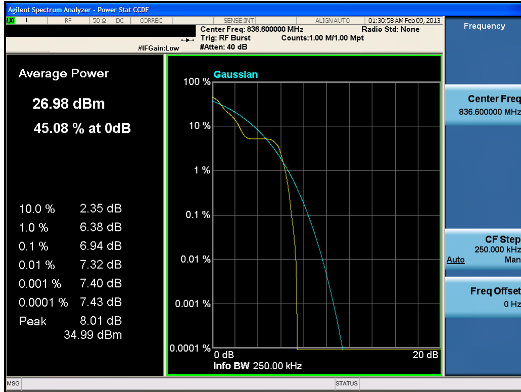
Plot 7-12. Peak-Average Ratio Plot (EDGE850 Mode – Ch. 190)
