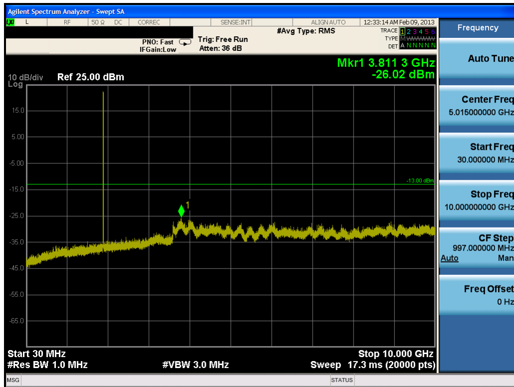
Plot 7-55. Conducted Spurious Plot (PCS WCDMA Mode – Ch. 9538)
