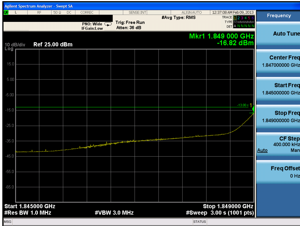
Plot 7-50. 4MHz Span Plot (PCS WCDMA Mode – Ch. 9262)
