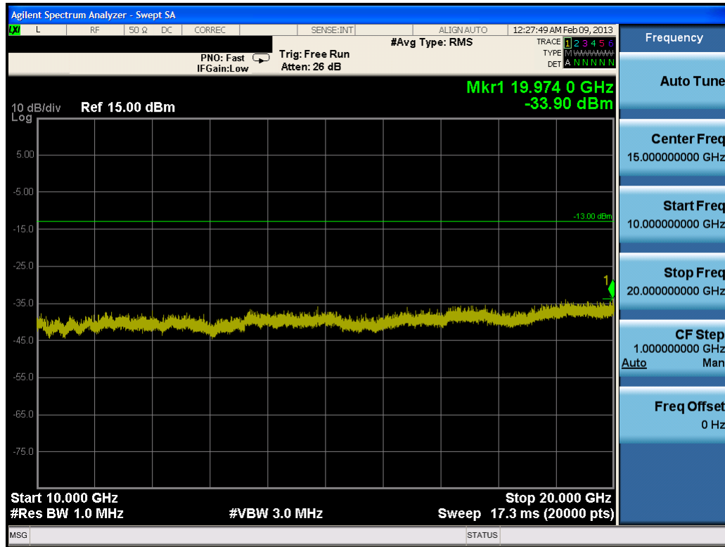
Plot 7-44. Conducted Spurious Plot (AWS WCDMA Mode – Ch. 1862)
