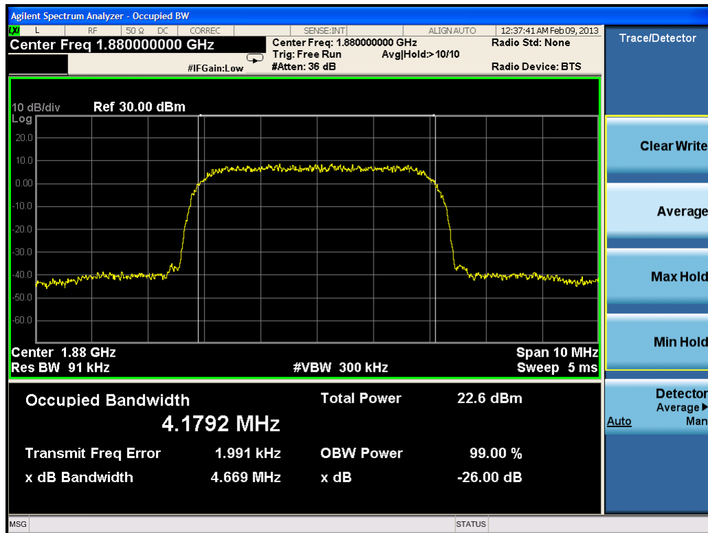
Plot 7-53. Occupied Bandwidth Plot (PCS WCDMA Mode – Ch. 9400)
