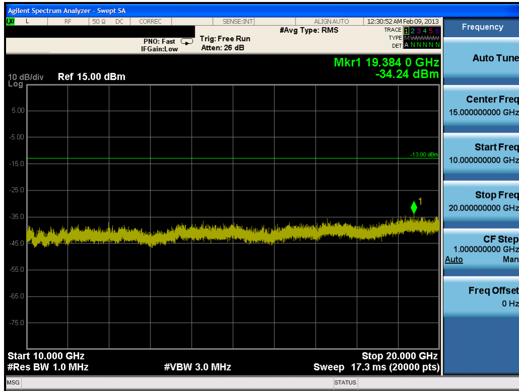
Plot 7-52. Conducted Spurious Plot (PCS WCDMA Mode – Ch. 9400)
