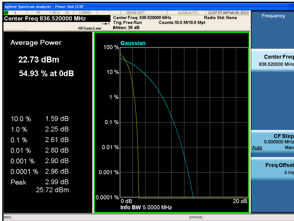
Plot 7-31. Peak-Average Ratio Plot (Cellular WCDMA Mode – Ch. 4183)
