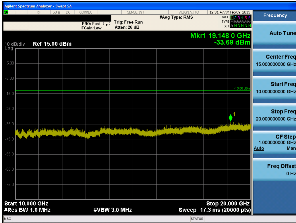
Plot 7-56. Conducted Spurious Plot (PCS WCDMA Mode – Ch. 9538)
