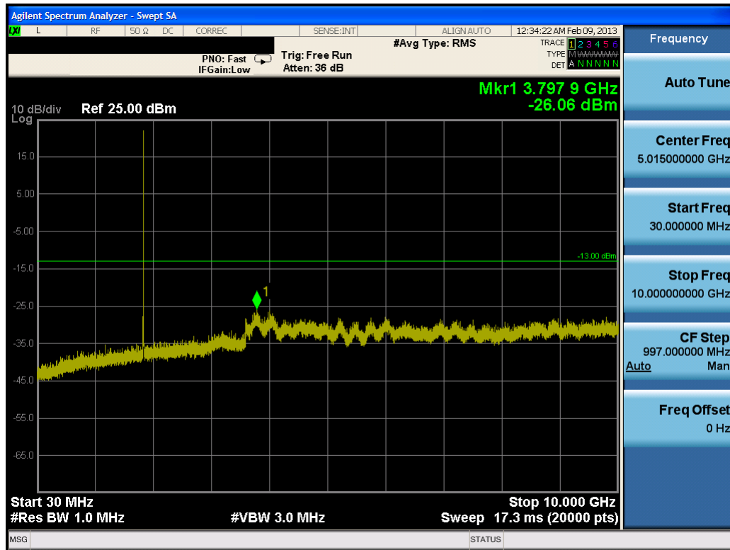
Plot 7-47. Conducted Spurious Plot (PCS WCDMA Mode – Ch. 9262)
