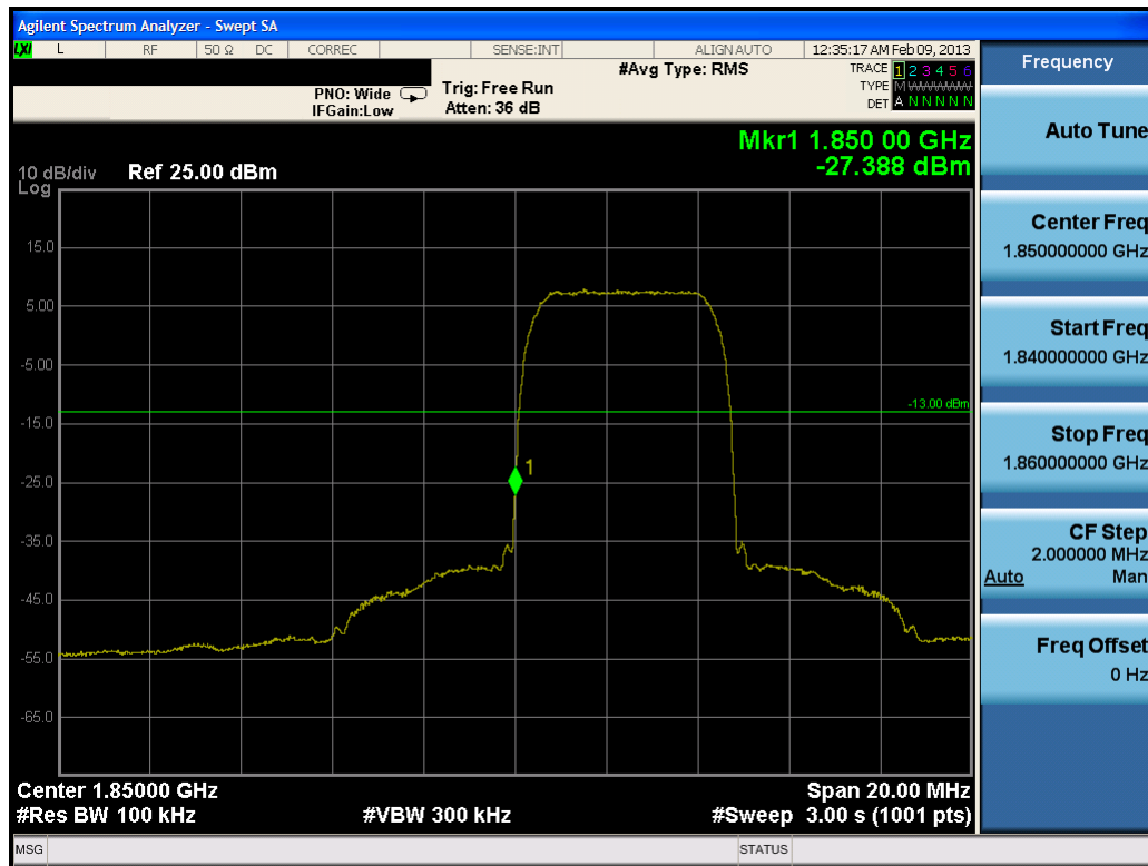
Plot 7-49. Band Edge Plot (PCS WCDMA Mode – Ch. 9262)
