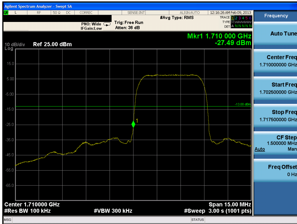
Plot 7-37. Band Edge Plot (AWS WCDMA Mode – Ch. 1312)
