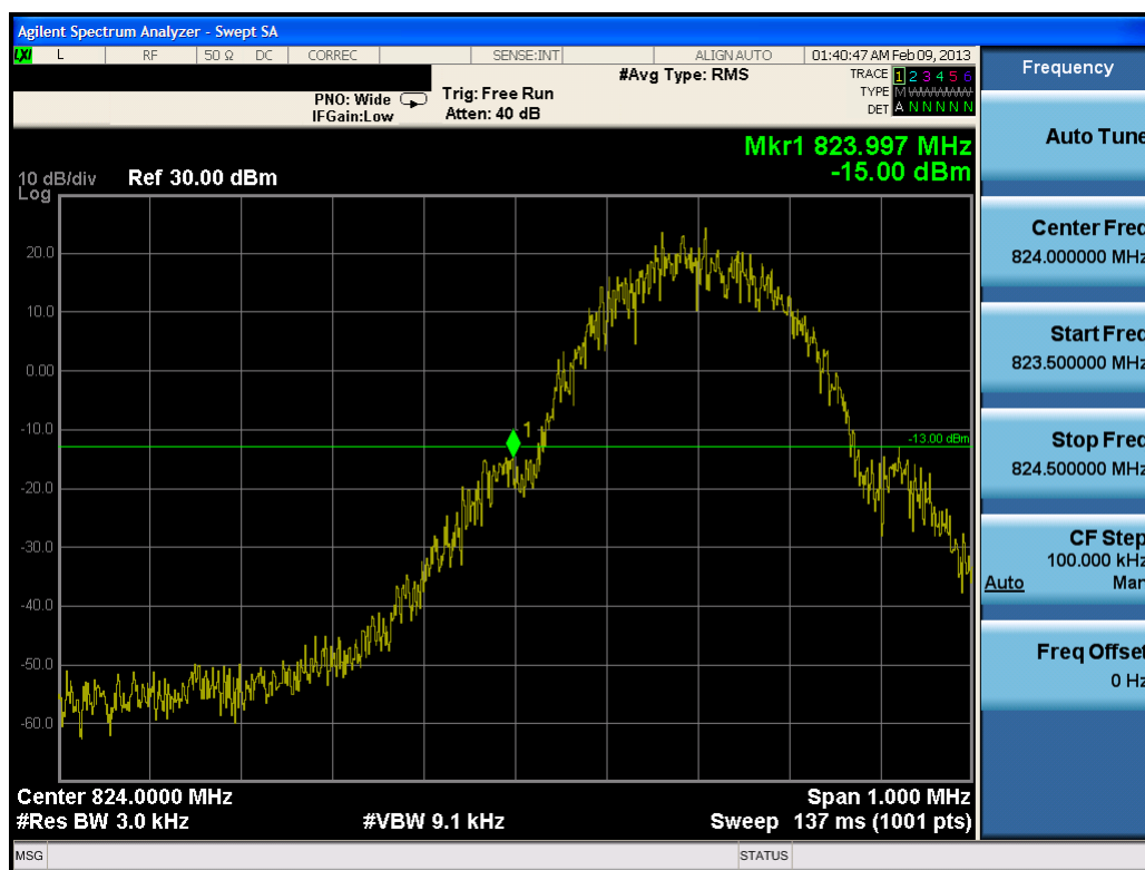
Plot 7-3. Band Edge Plot (Cellular GSM Mode – Ch. 128)
