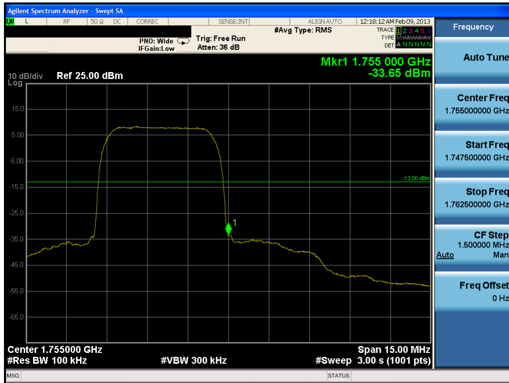
Plot 7-45. Band Edge Plot (AWS WCDMA Mode – Ch. 1862)
