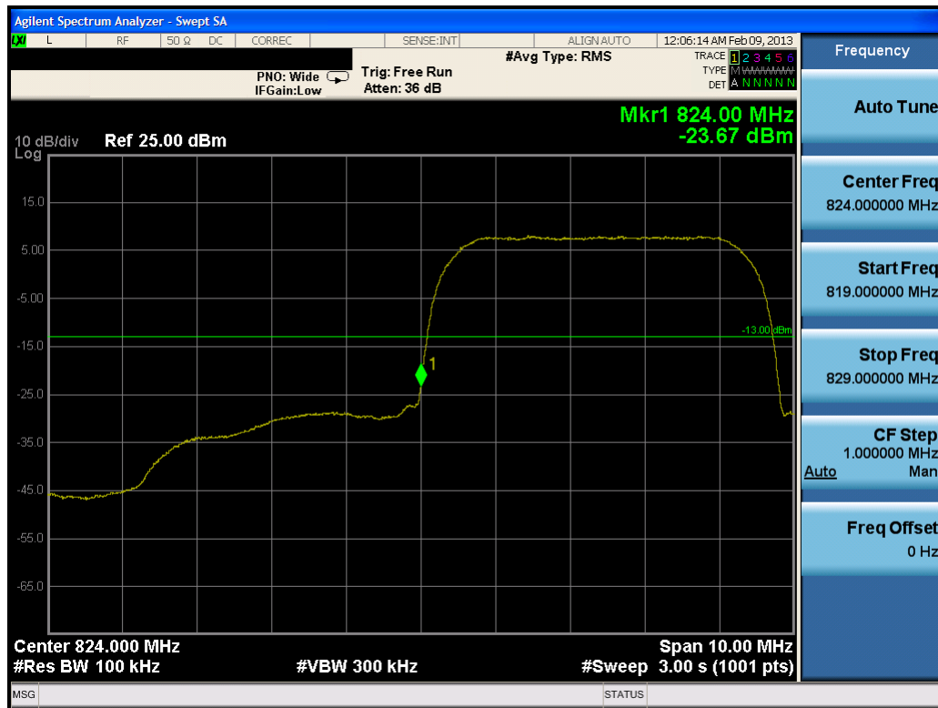
Plot 7-27. Band Edge Plot (Cellular WCDMA Mode – Ch. 4132)
