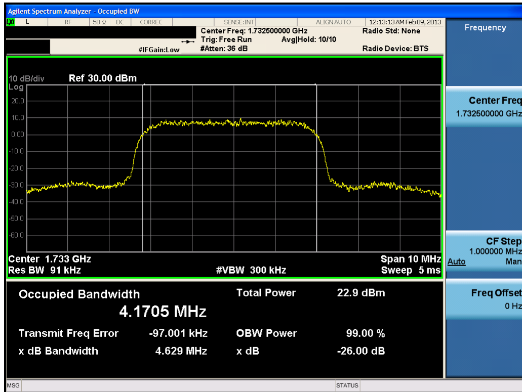
Plot 7-41. Occupied Bandwidth Plot (AWS WCDMA Mode – Ch. 1412)
