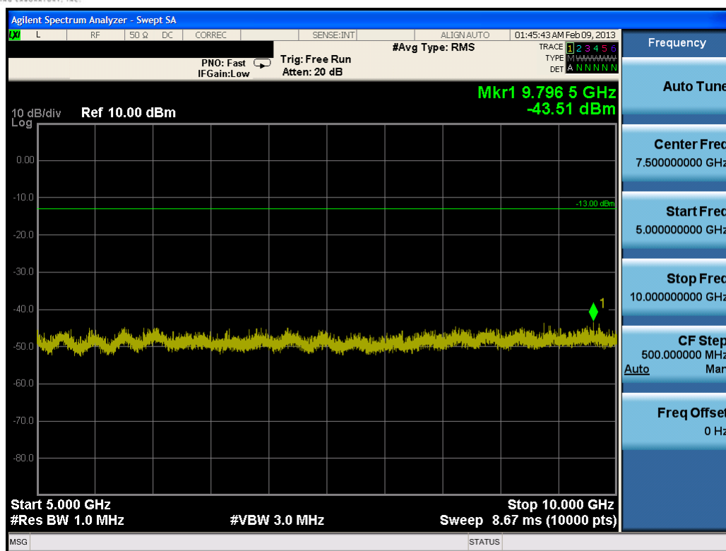
Plot 7-2. Conducted Spurious Plot (Cellular GSM Mode – Ch. 128)
