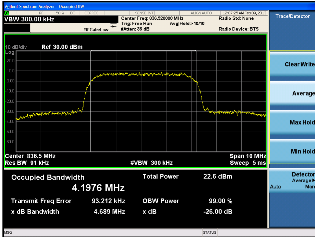
Plot 7-30. Occupied Bandwidth Plot (Cellular WCDMA Mode – Ch. 4183)
