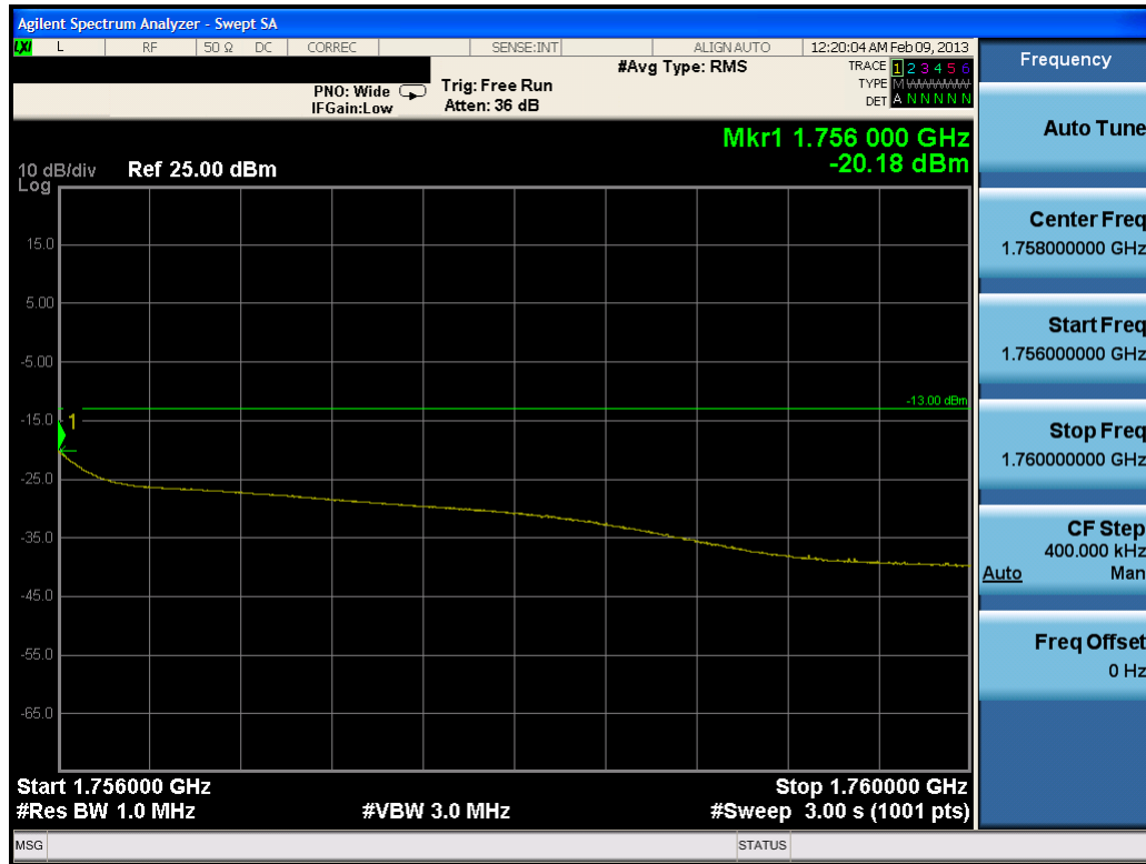
Plot 7-46. 4MHz Span Plot (AWS WCDMA Mode – Ch. 1862)
