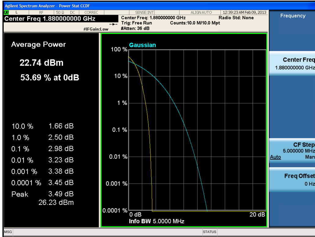
Plot 7-54. Peak-Average Ratio Plot (PCS WCDMA Mode – Ch. 9400)
