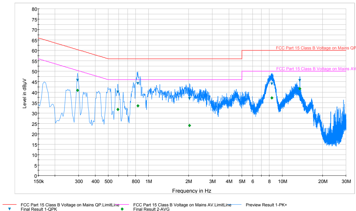
Plot 8-2. Line-Conducted Test Plot (N)
