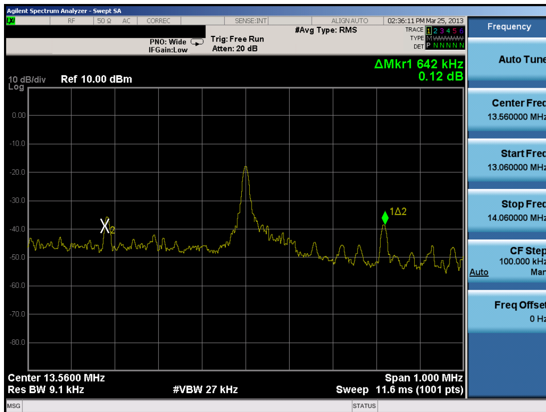
Figure 8-3. 20dB Bandwidth Plot (Wireless Charging Cover)
