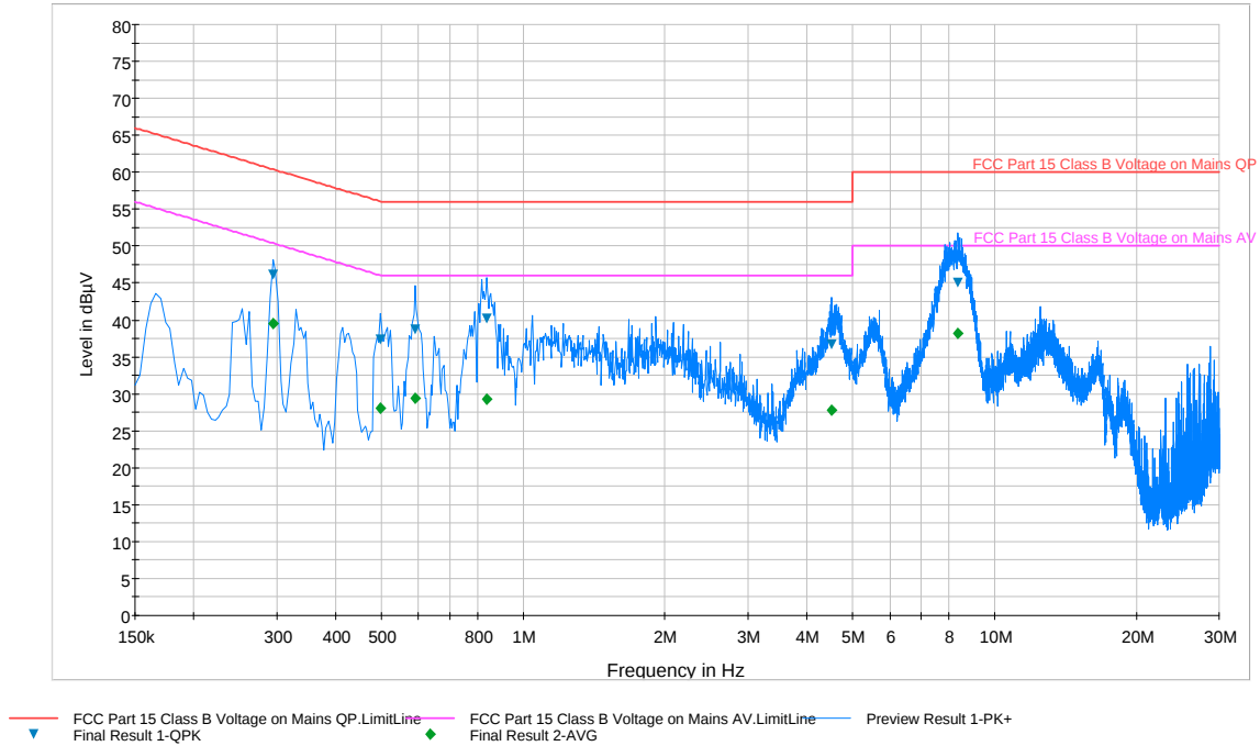
Plot 6-101. Line Conducted Plot with 802.11a UNII Band 1 (L1)
