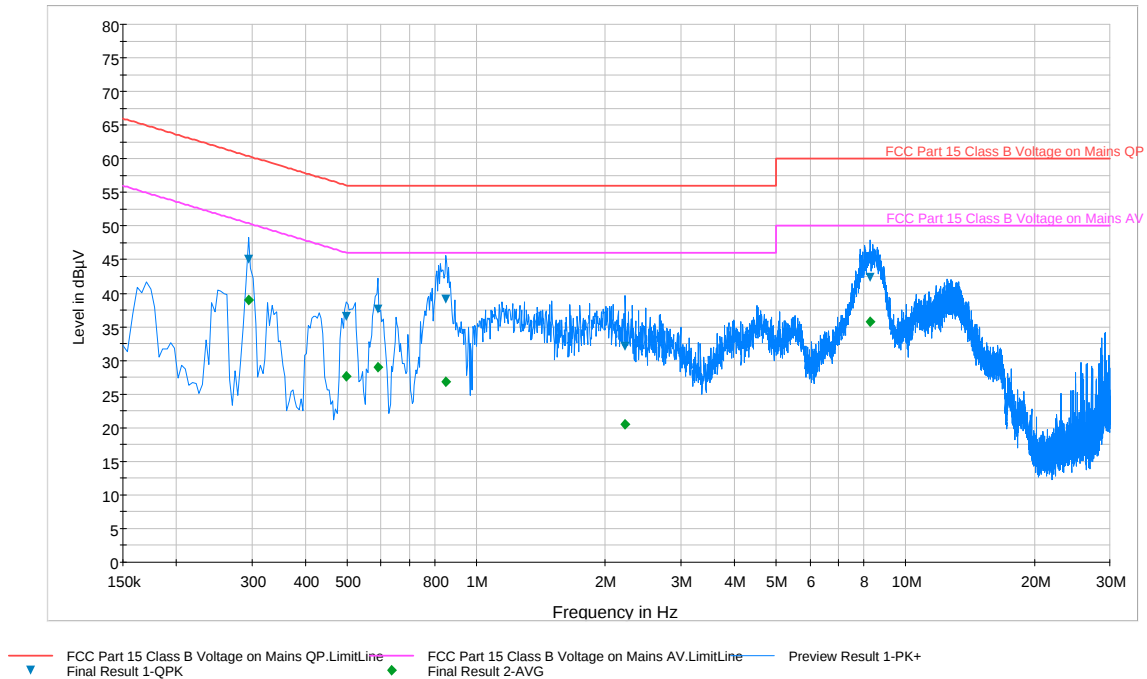
Plot 6-105. Line Conducted Plot with 802.11a UNII Band 3 (L1)
