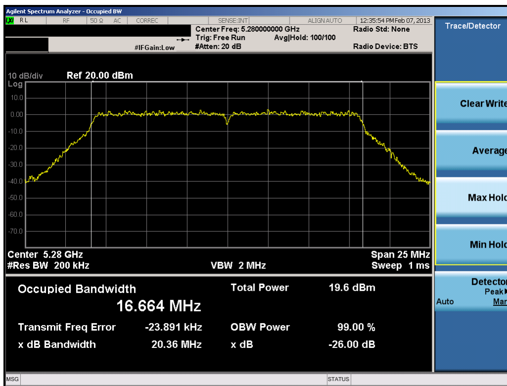
Plot 6-10. 26dB Bandwidth Plot (802.11a (UNII Band 2) – Ch. 56)
