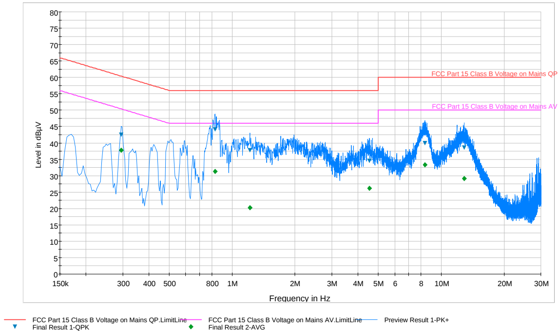
Plot 6-102. Line Conducted Plot with 802.11a UNII Band 1 (N)
