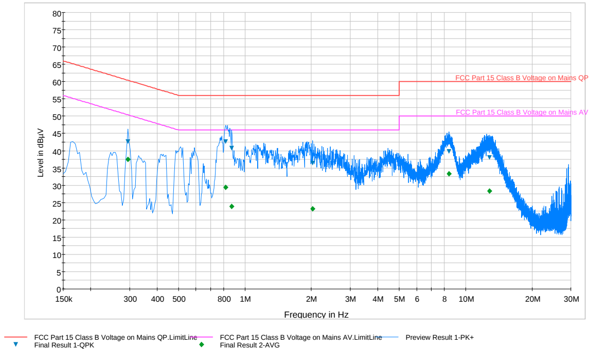
Plot 6-104. Line Conducted Plot with 802.11a UNII Band 2 (N)
