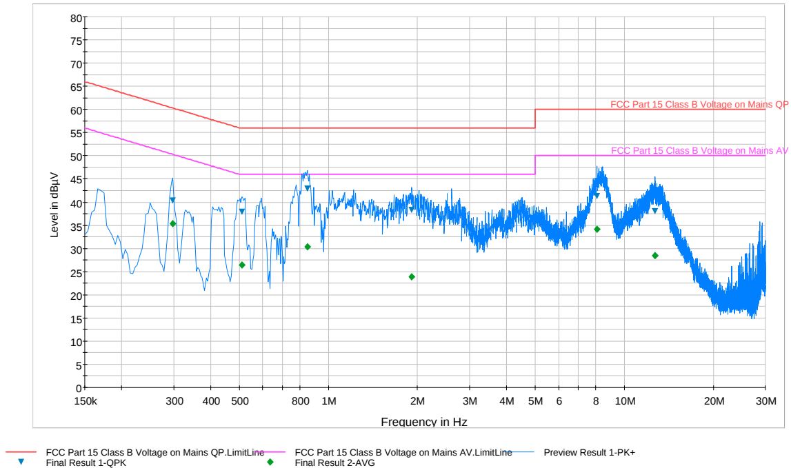
Plot 6-106. Line Conducted Plot with 802.11a UNII Band 3 (N)
