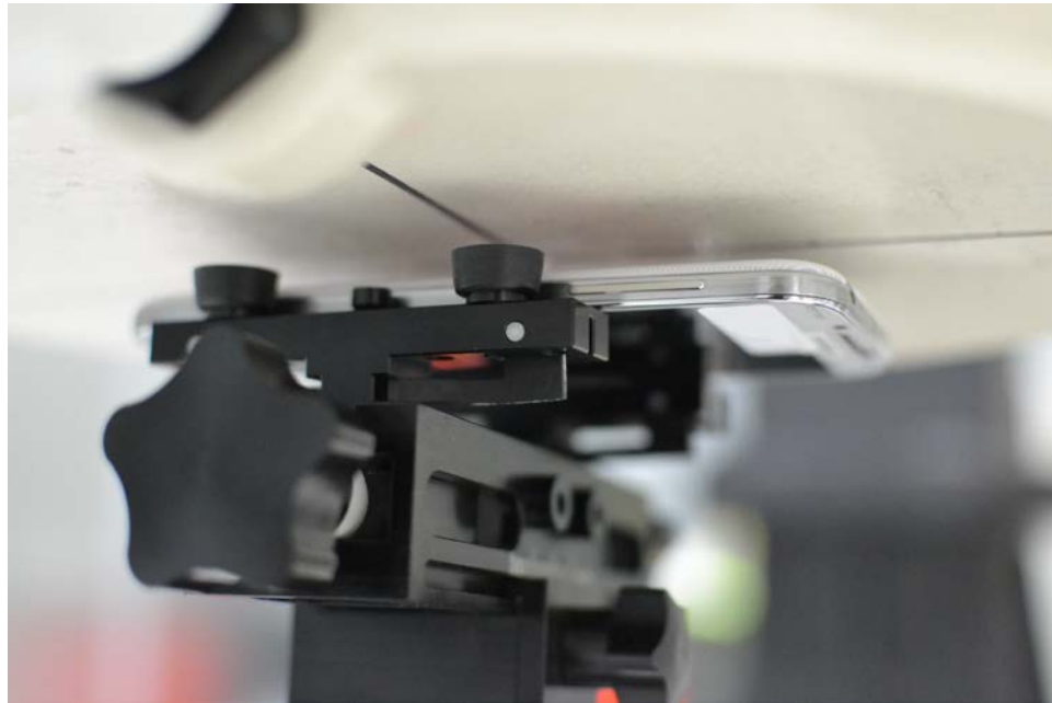
SAR Test Setup Photo 1: Back at 1.0 cm
