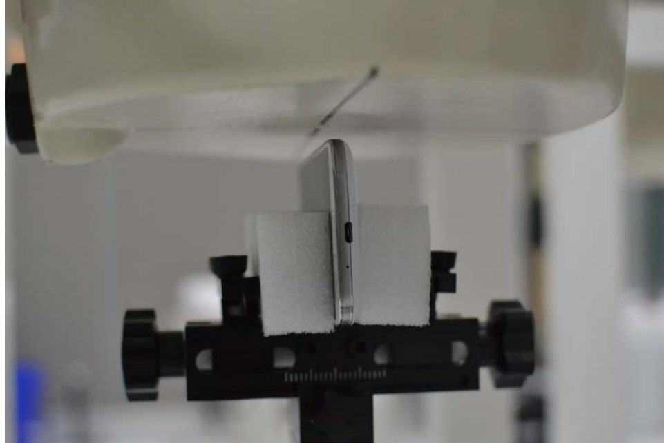
SAR Test Setup Photo 5: Right with Wireless Charging Cover at 1.0 cm
