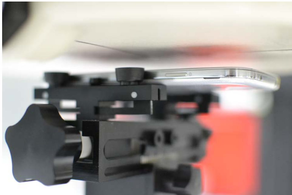
SAR Test Setup Photo 2: Front at 1.0 cm
