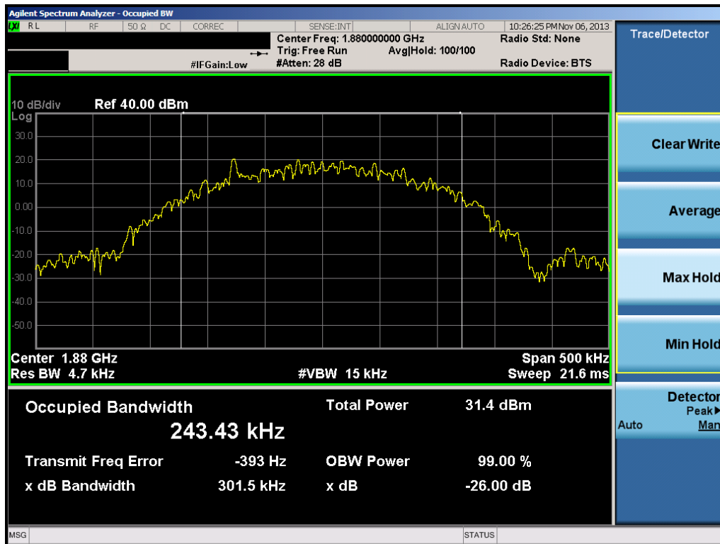
Plot 6-4. Occupied Bandwidth Plot (EDGE1900 Mode – Ch. 661)
