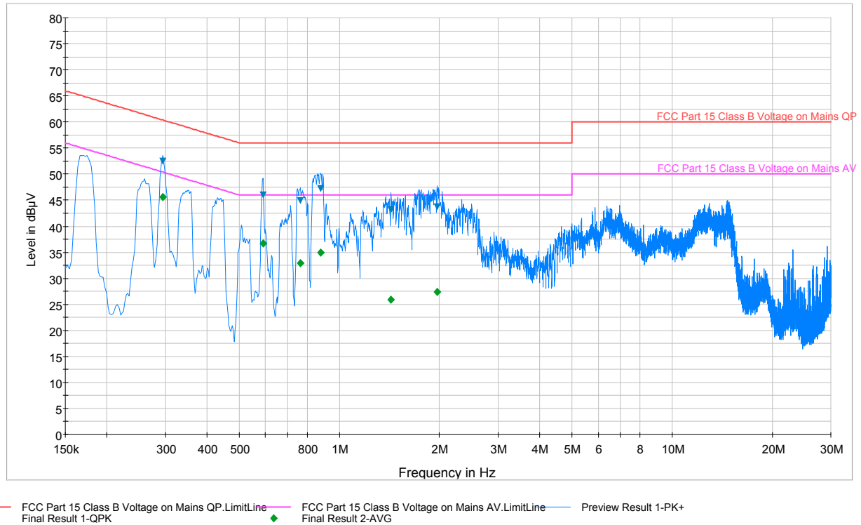
Plot 6-5. Line-Conducted Test Plot (L1)
