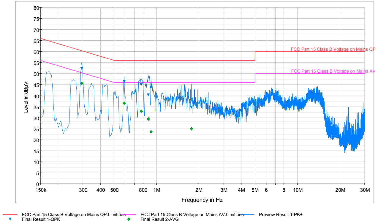
Plot 6-6. Line-Conducted Test Plot (N)
