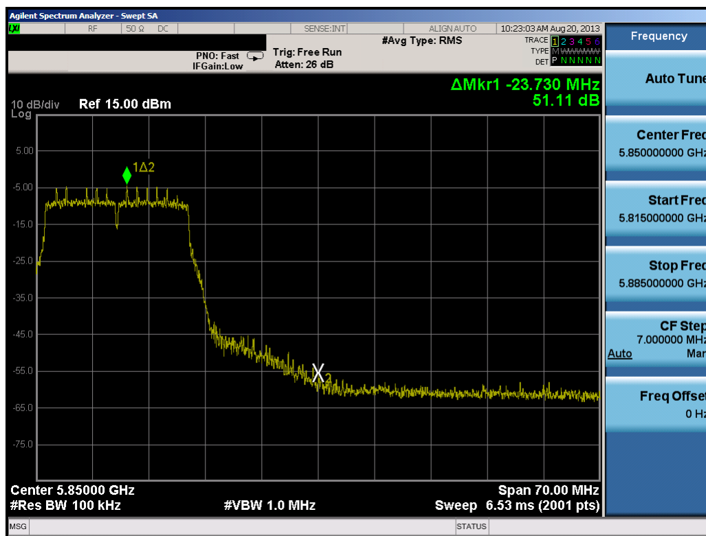
Plot 6-46. Band Edge Plot (20MHz BW 802.11n (5.8GHz) – Ch. 165)
