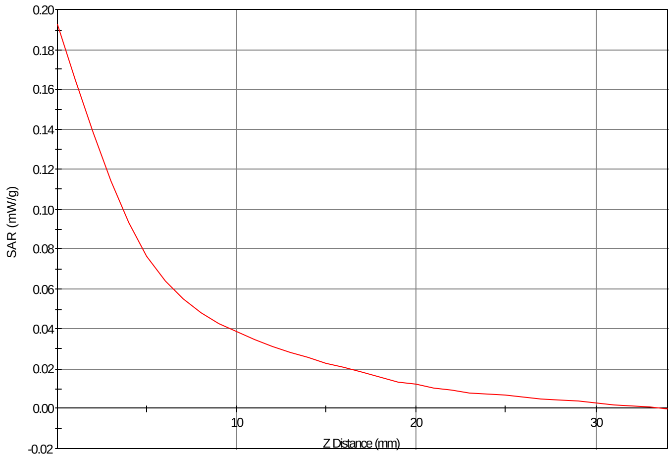
SAR - Z Axis at Hotspot x:-5.0 y:15.0
