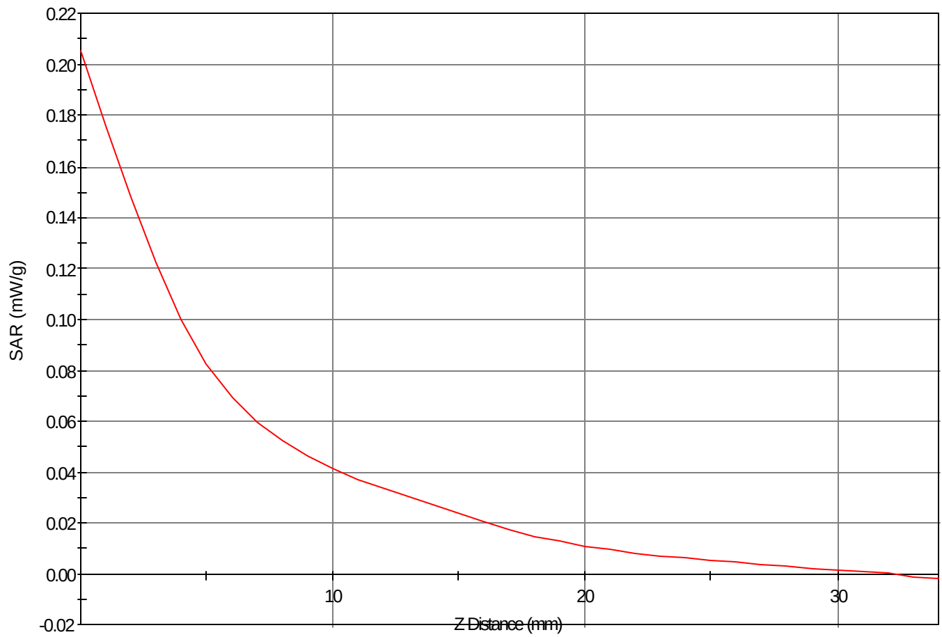
SAR - Z Axis at Hotspot x:-12.0 y:14.0
