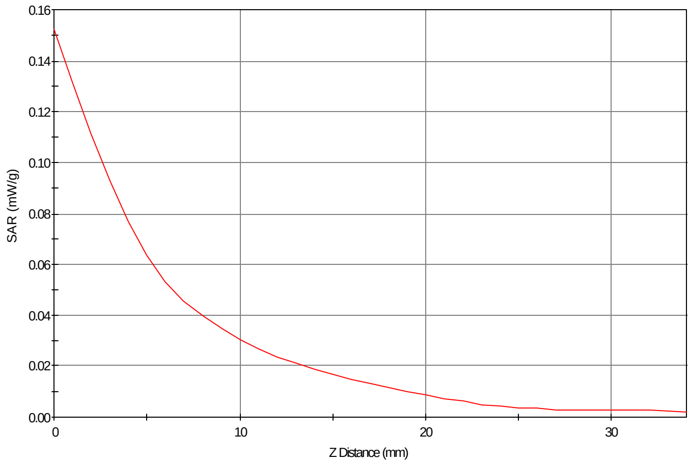
SAR - Z Axis at Hotspot x:-7.0 y:18.0
