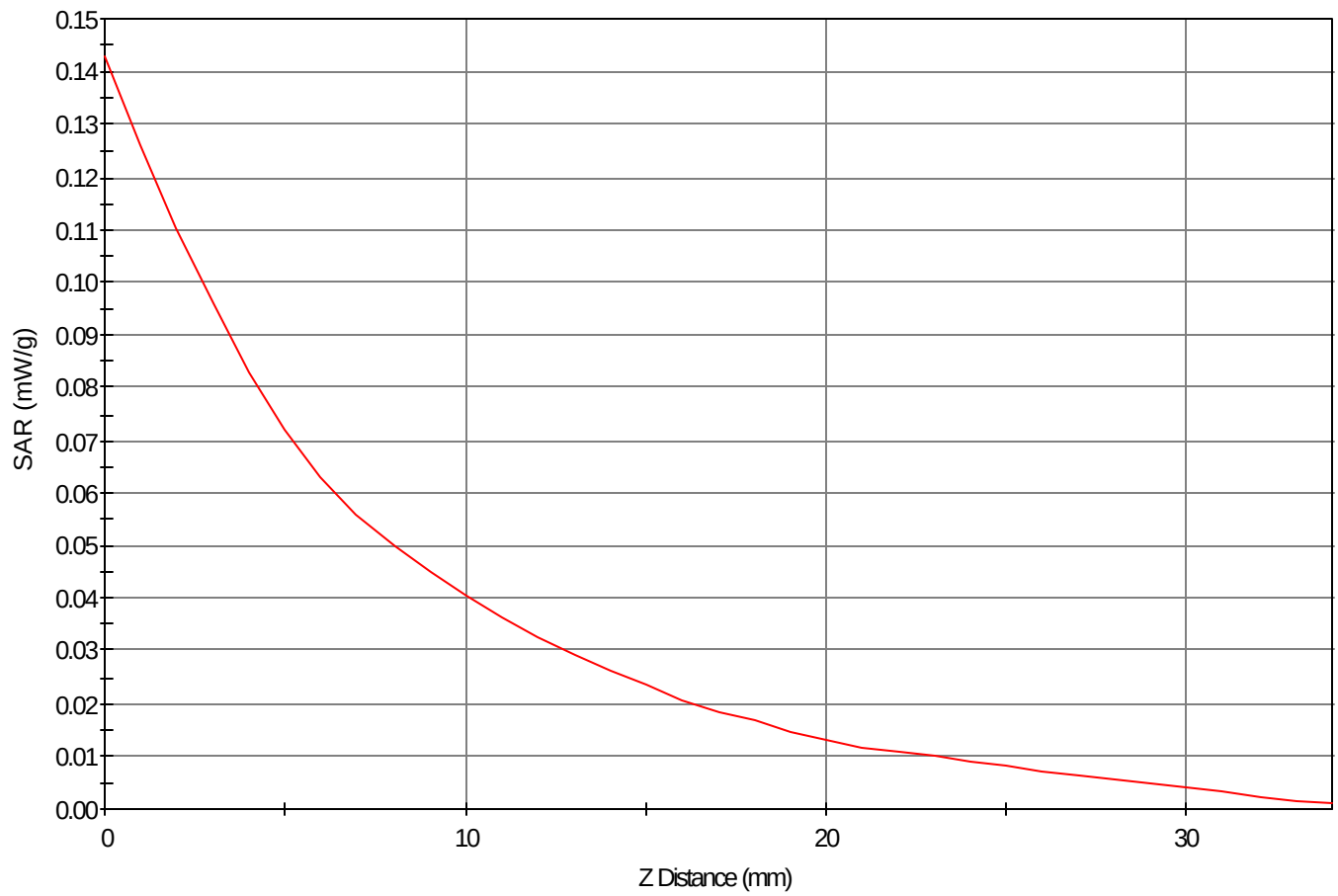
SAR - Z Axis at Hotspot x:42.0 y:0.0
