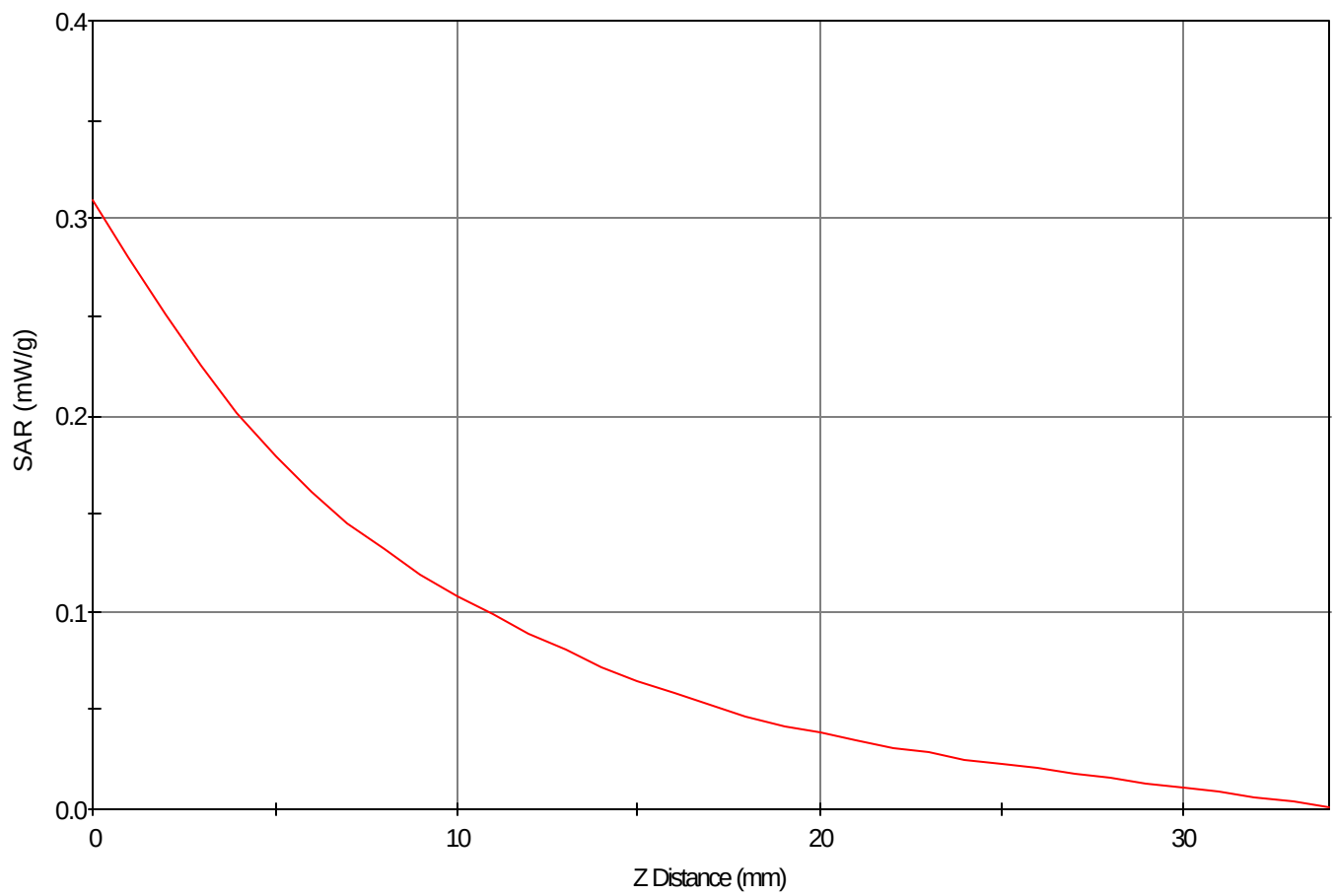
SAR - Z Axis at Hotspot x:20.0 y:-8.0
