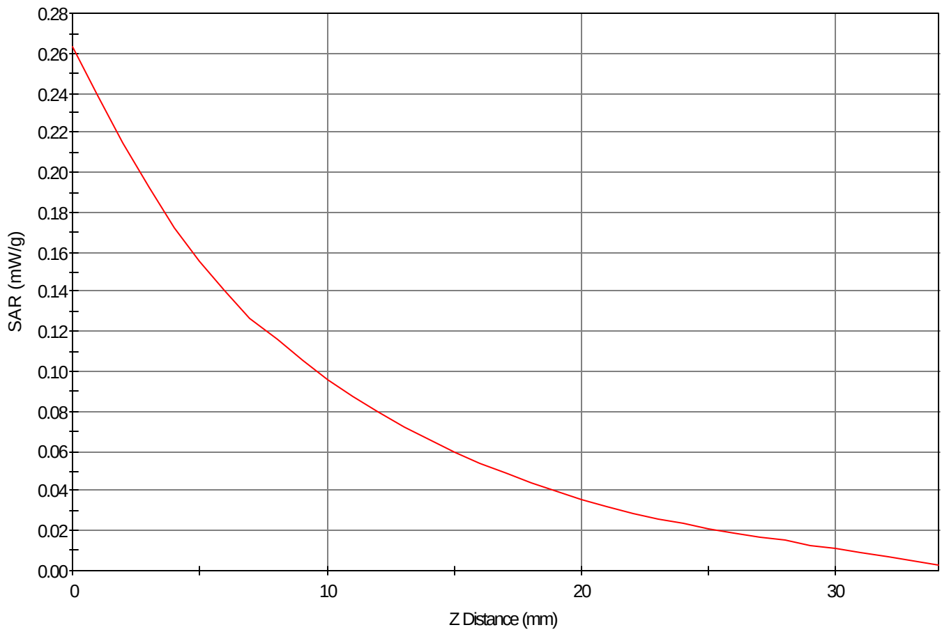
SAR - Z Axis at Hotspot x:25.0 y:-10.0
