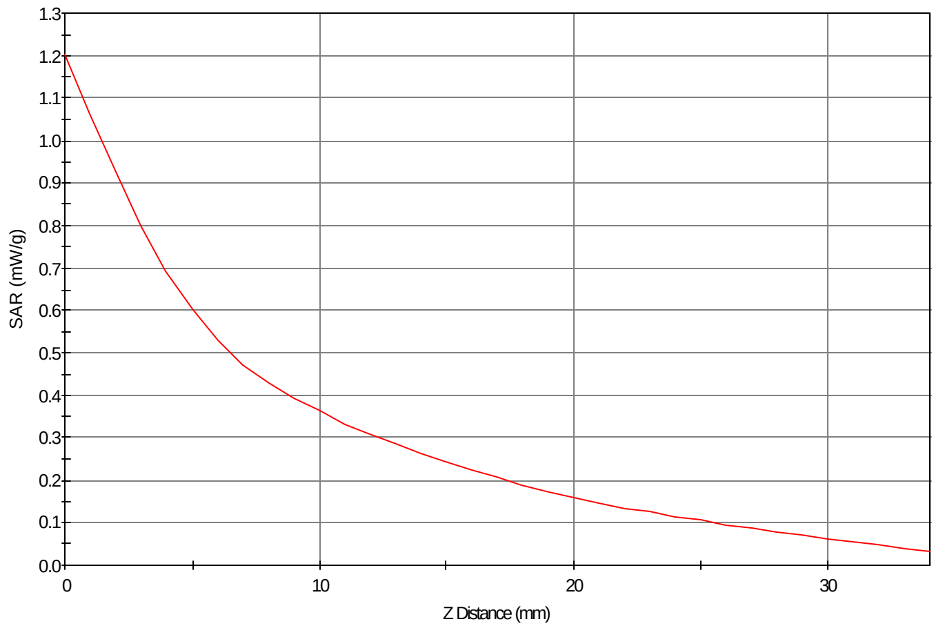
SAR - Z Axis at Hotspot x:2.0 y:-18.0
