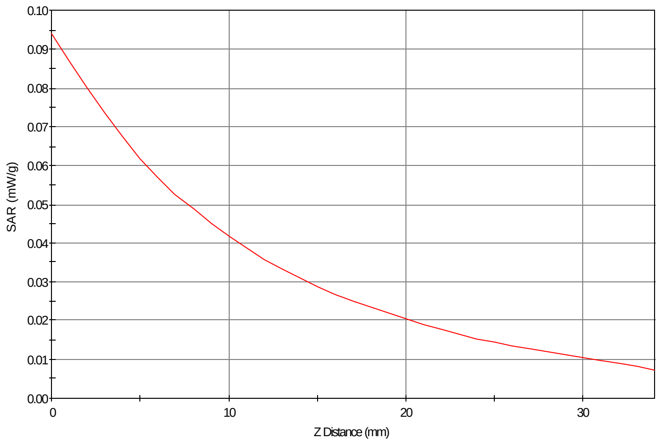
SAR - Z Axis at Hotspot x:41.0 y:-3.0
