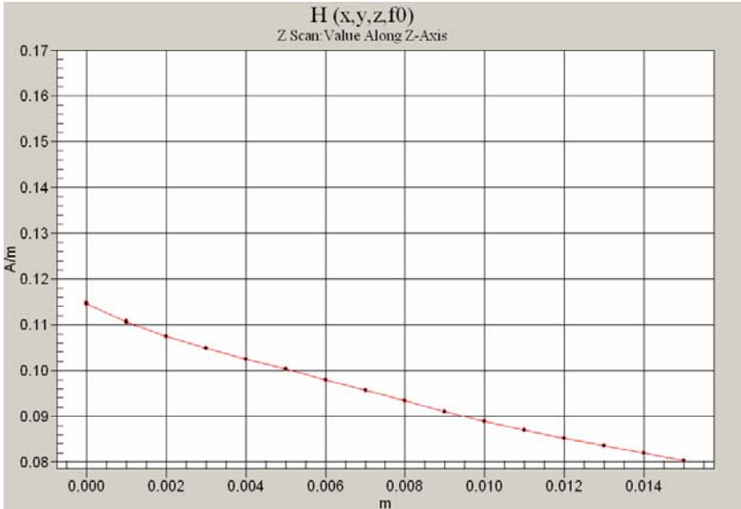
Figure 7 Z-Axis Scan at maximum point above a typical wireless device for H-field
