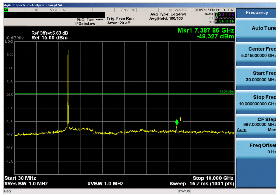
Plot 6-20. Conducted Spurious Plot (802.11b – Ch. 11)
