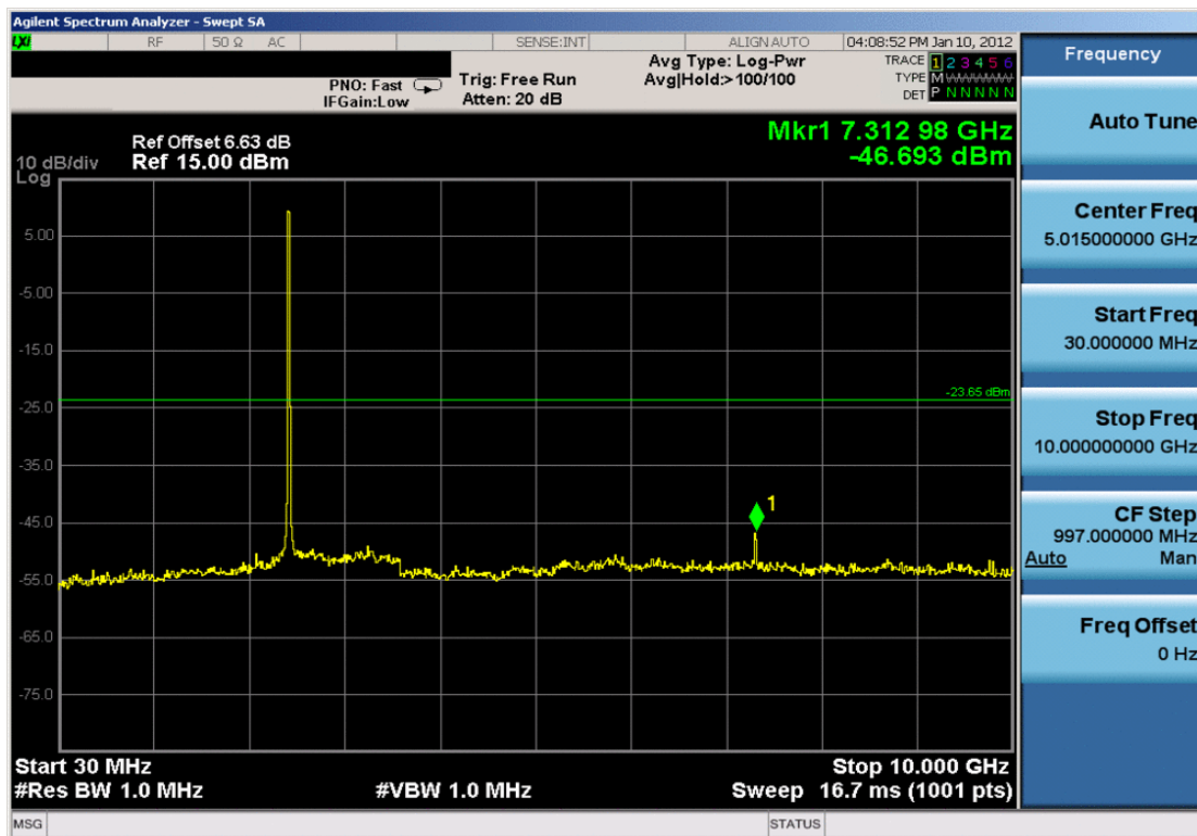
Plot 6-18. Conducted Spurious Plot (802.11b – Ch. 6)
