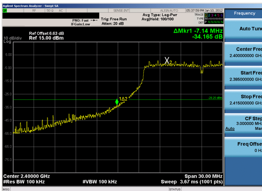
Plot 6-14. Band Edge Plot (802.11g – Ch. 1)
