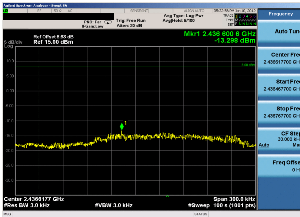
Plot 6-11. Power Spectral Density Plot (802.11g – Ch. 6)
