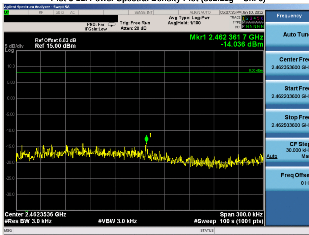
Plot 6 11. Power Spectral Density Plot (802.11g – Ch. 11)
