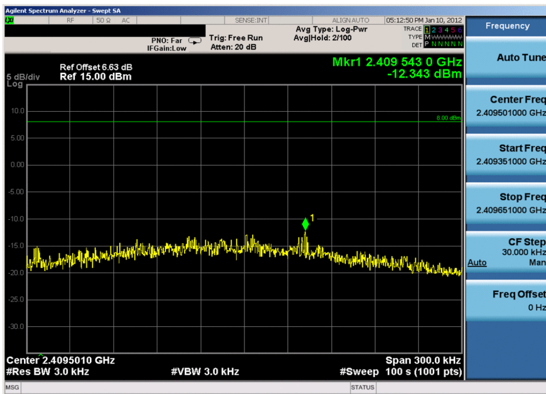
Plot 6-10. Power Spectral Density Plot (802.11g - Ch. 1)
