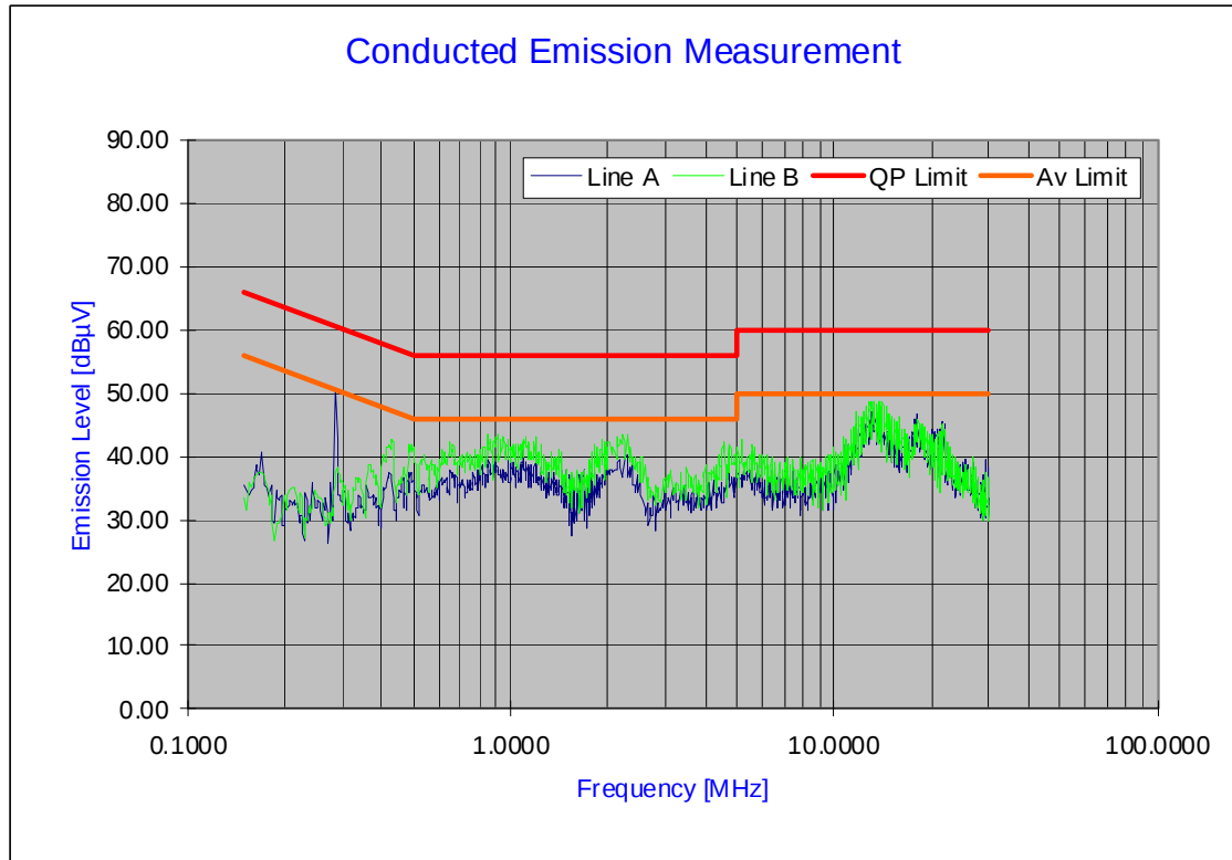
Plot 6-23. Line Conducted Plot with 802.11g
