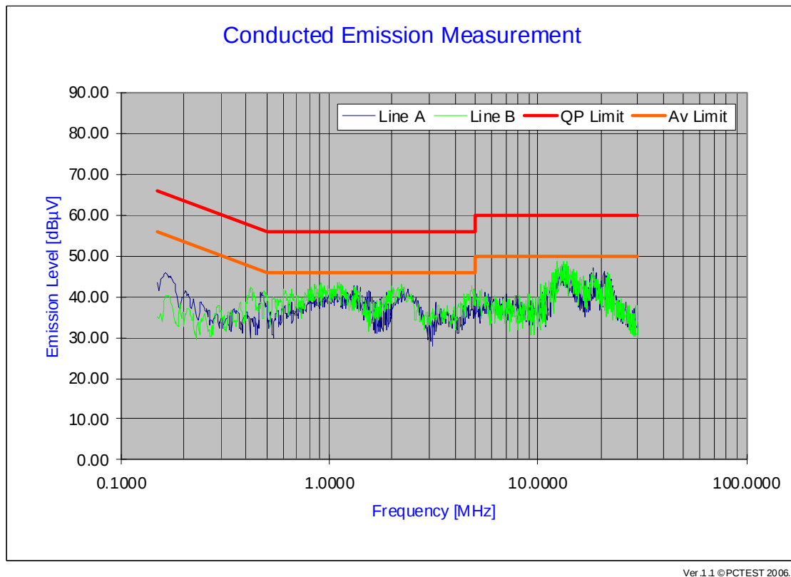
Plot 6-22. Line Conducted Plot with 802.11b
