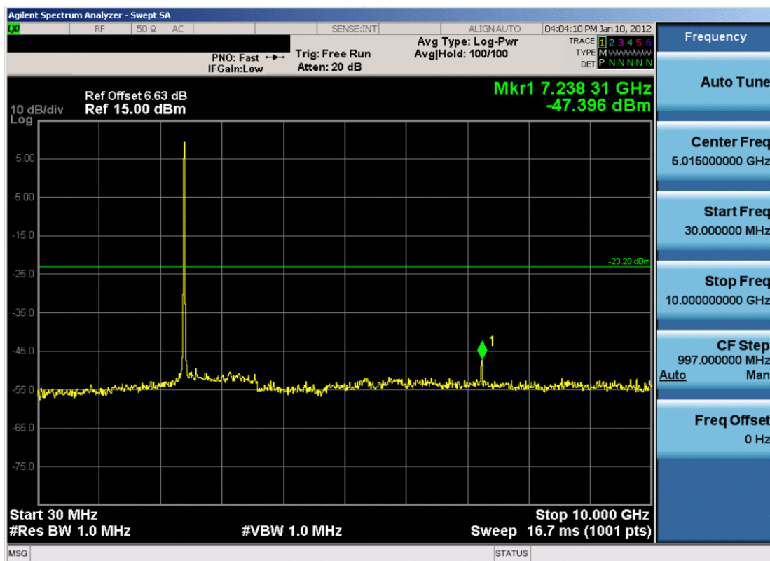
Plot 6-16. Conducted Spurious Plot (802.11b – Ch. 1)
