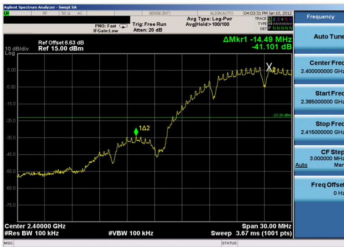
Plot 6-12. Band Edge Plot (802.11b – Ch. 1)
