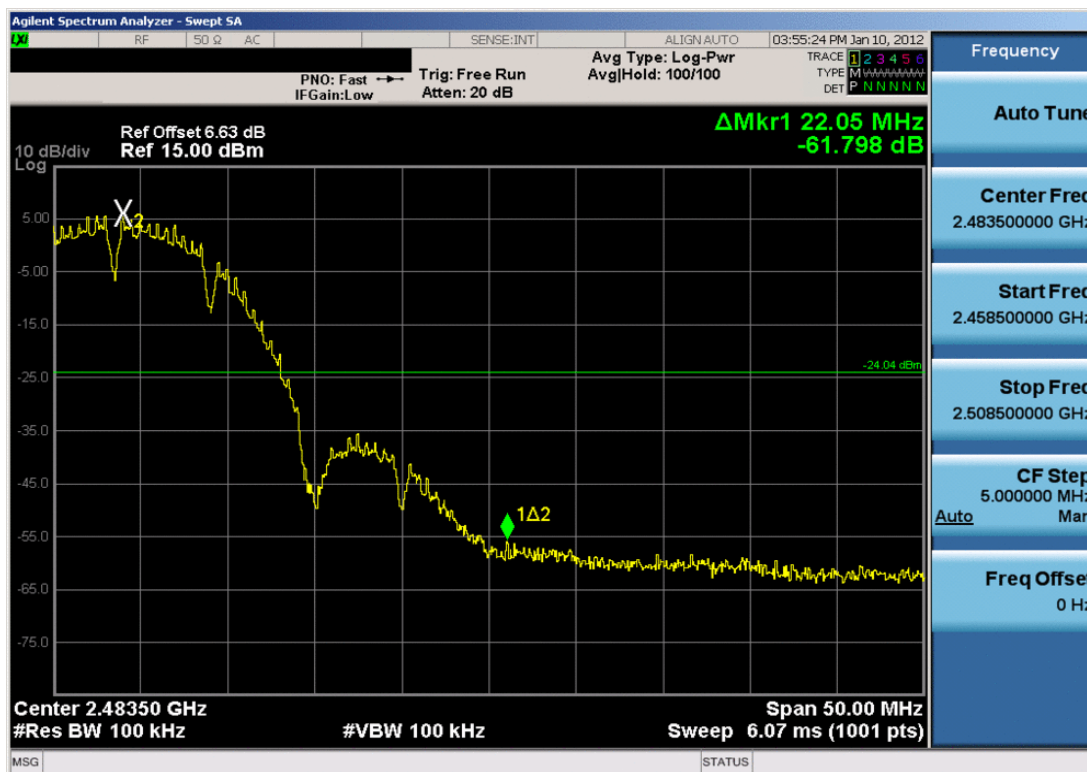
Plot 6-13. Band Edge Plot (802.11b – Ch. 11)
