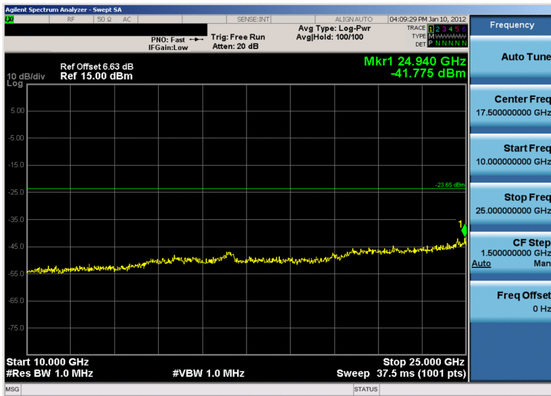
Plot 6-19. Conducted Spurious Plot (802.11b – Ch. 6)
