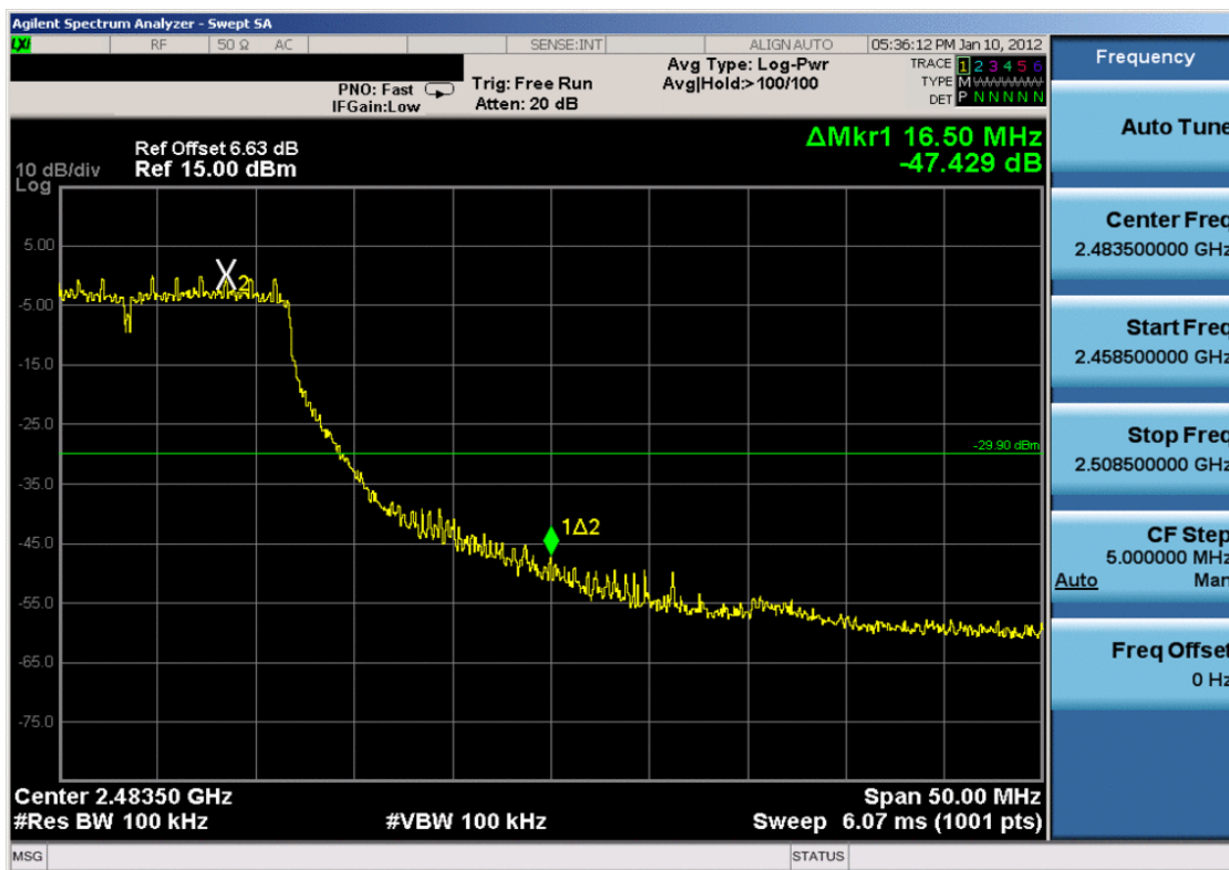
Plot 6-15. Band Edge Plot (802.11g – Ch. 11)
