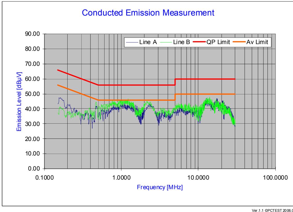
Plot 6-22. Line Conducted Plot with Bluetooth
