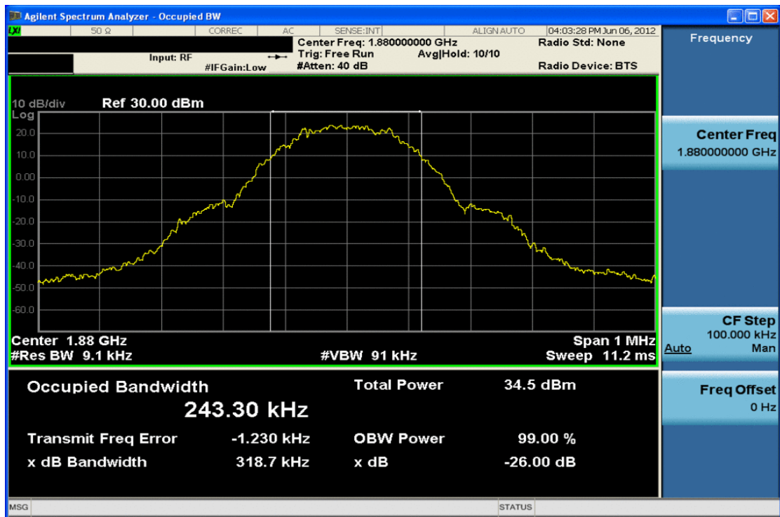
Plot 7-16. Occupied Bandwidth Plot (PCS GSM Mode – Ch. 661)
