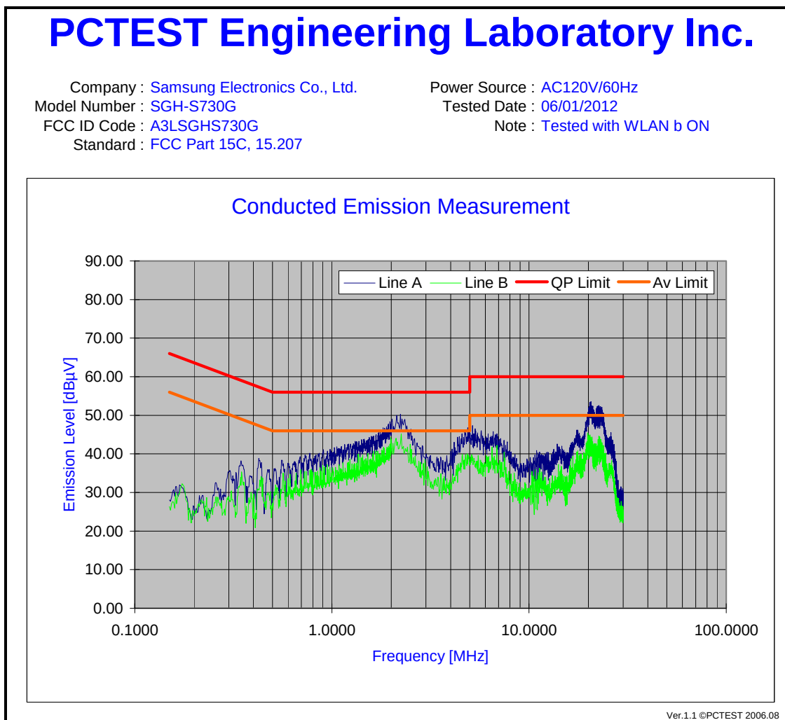
Plot 6-31. Line Conducted Plot with 802.11b
