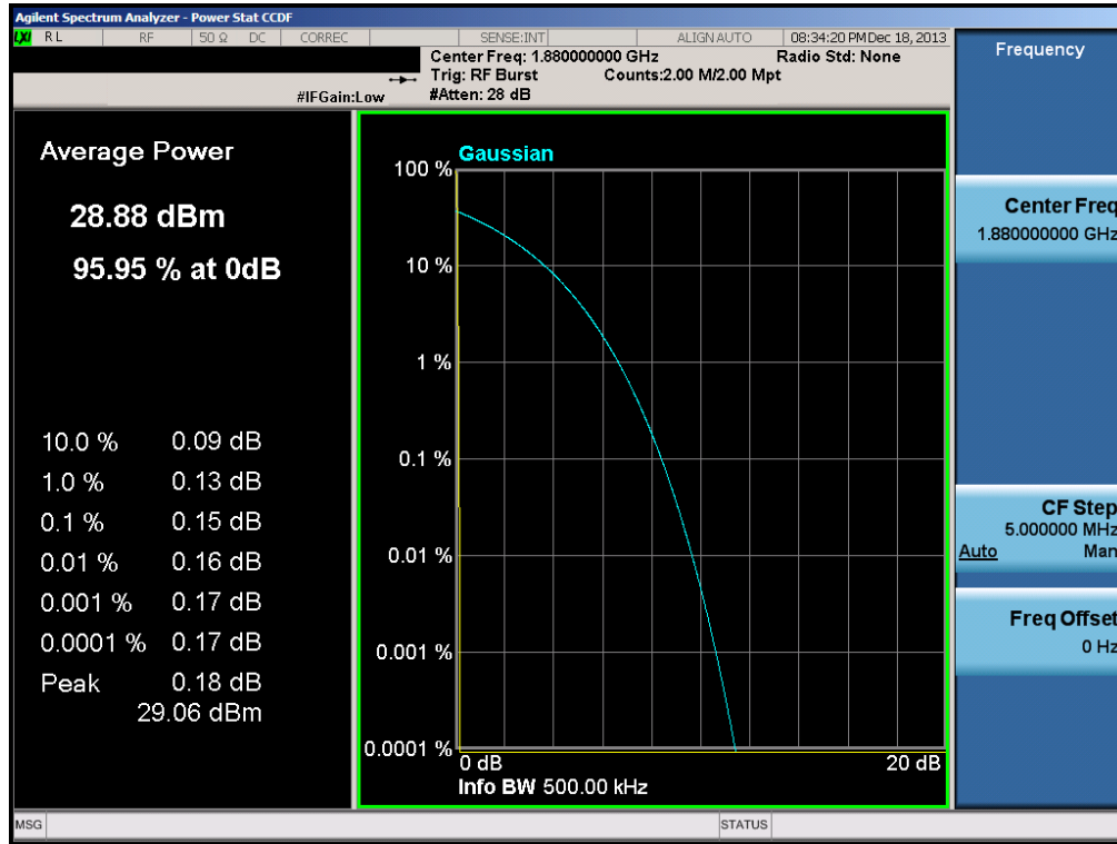
Plot 6-46. Peak-Average Ratio Plot (PCS GSM Mode – Ch. 661)
