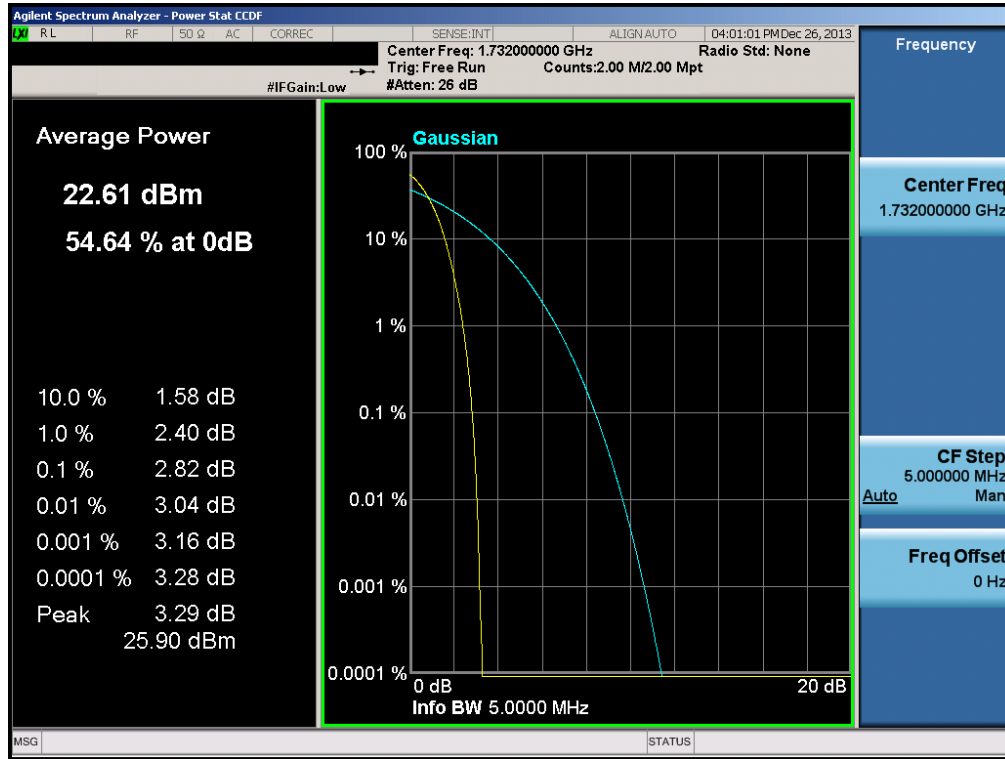
Plot 6-48. Peak-Average Ratio Plot (AWS WCDMA Mode – Ch. 1412)
