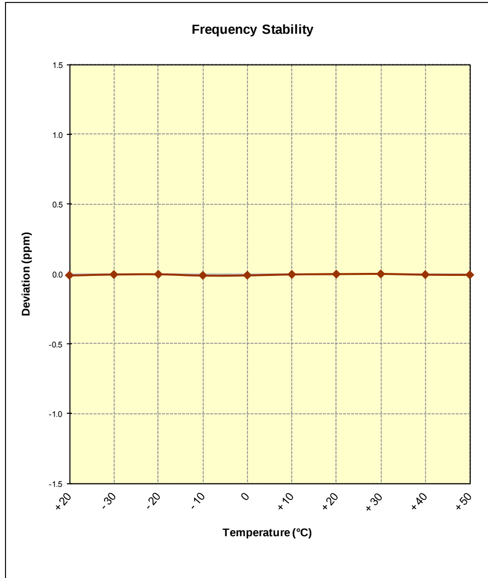
Figure 6-8. Frequency Stability Graph (AWS WCDMA Mode – Ch. 1413)
