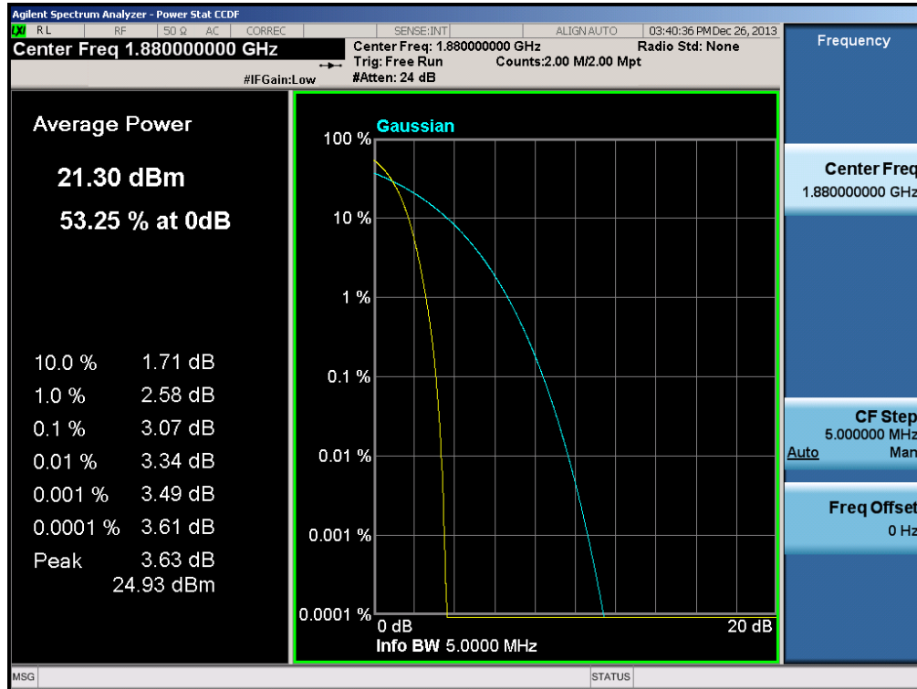
Plot 6-49. Peak-Average Ratio Plot (PCS WCDMA Mode – Ch. 9400)
