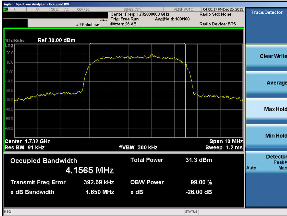
Plot 6-5. Occupied Bandwidth Plot (AWS WCDMA Mode – Ch. 1412)
