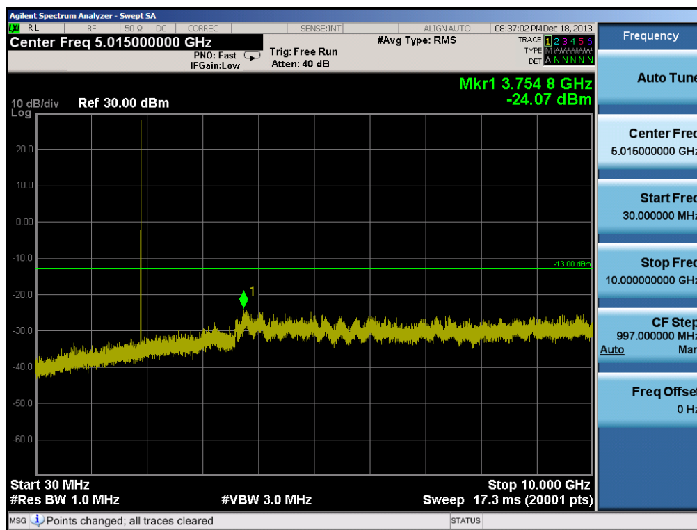
Plot 6-20. Conducted Spurious Plot (PCS GSM Mode – Ch. 810)
