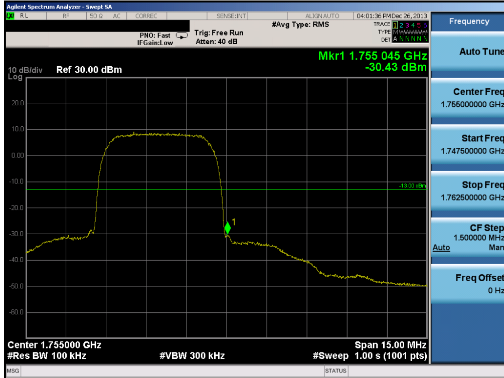
Plot 6-40. Band Edge Plot (AWS WCDMA Mode – Ch. 1862)
