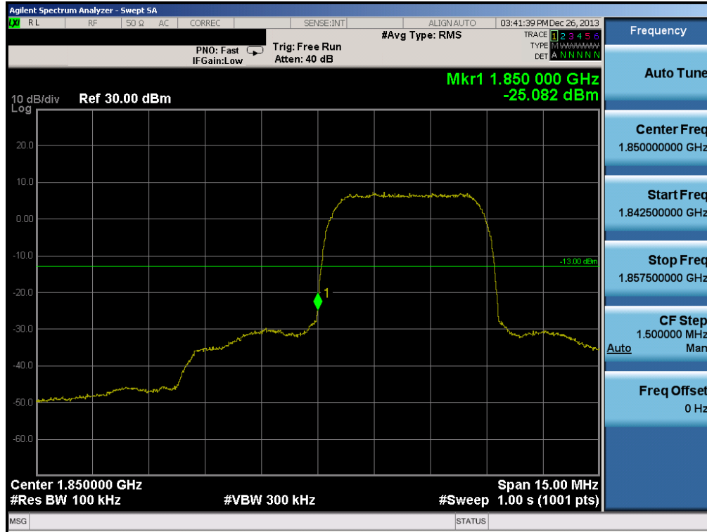
Plot 6-42. Band Edge Plot (PCS WCDMA Mode – Ch. 9262)
