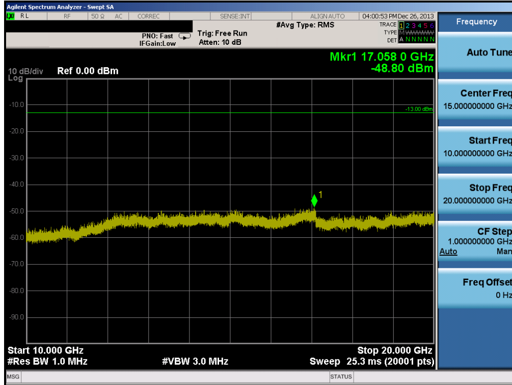
Plot 6-25. Conducted Spurious Plot (AWS WCDMA Mode – Ch. 1412)
