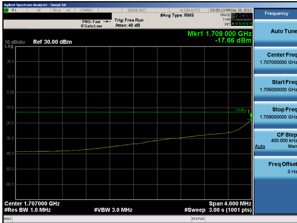
Plot 6-39. 4MHz Span Plot (AWS WCDMA Mode – Ch. 1312)
