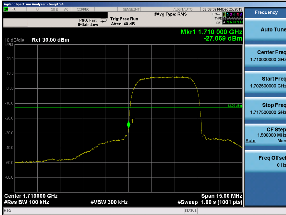
Plot 6-38. Band Edge Plot (AWS WCDMA Mode – Ch. 1312)
