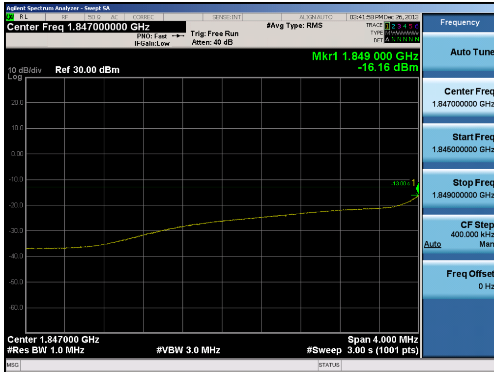
Plot 6-43. 4MHz Span Plot (PCS WCDMA Mode – Ch. 9262)
