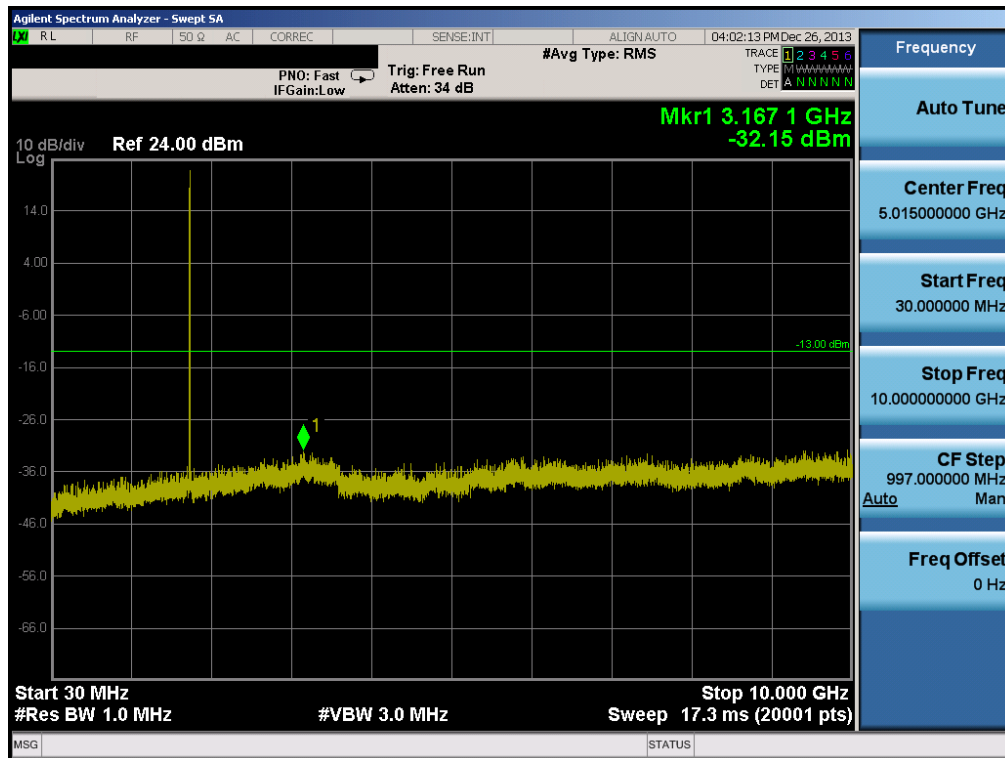
Plot 6-26. Conducted Spurious Plot (AWS WCDMA Mode – Ch. 1862)
