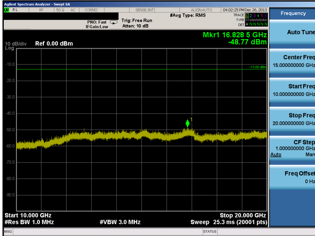
Plot 6-27. Conducted Spurious Plot (AWS WCDMA Mode – Ch. 1862)
