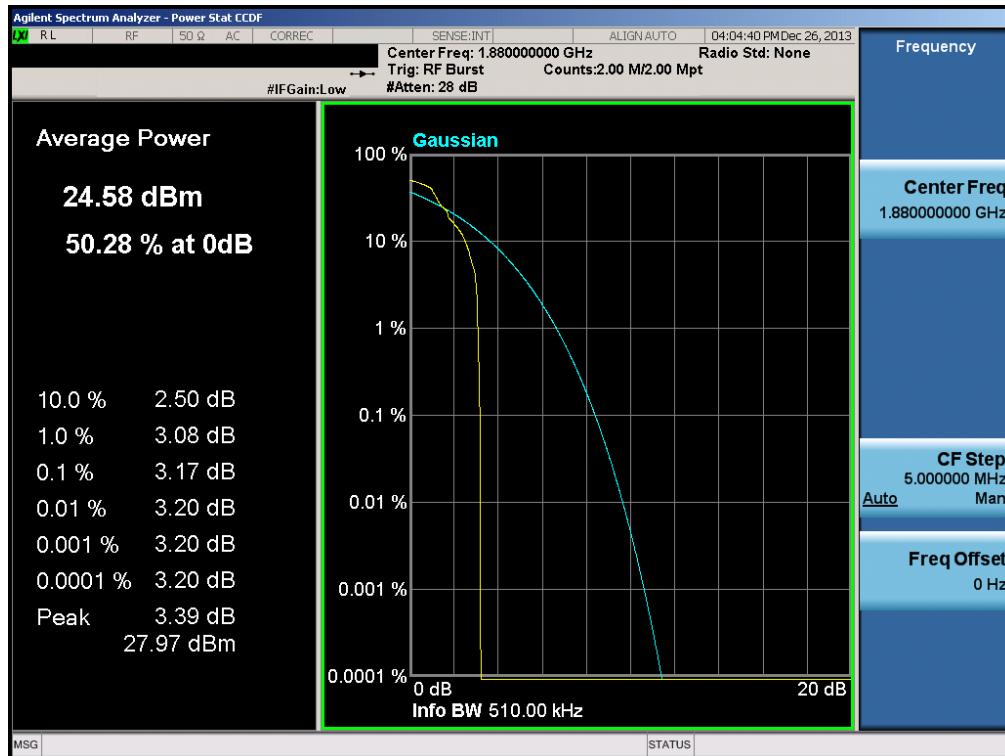
Plot 6-47. Peak-Average Ratio Plot (EDGE1900 Mode – Ch. 661)
