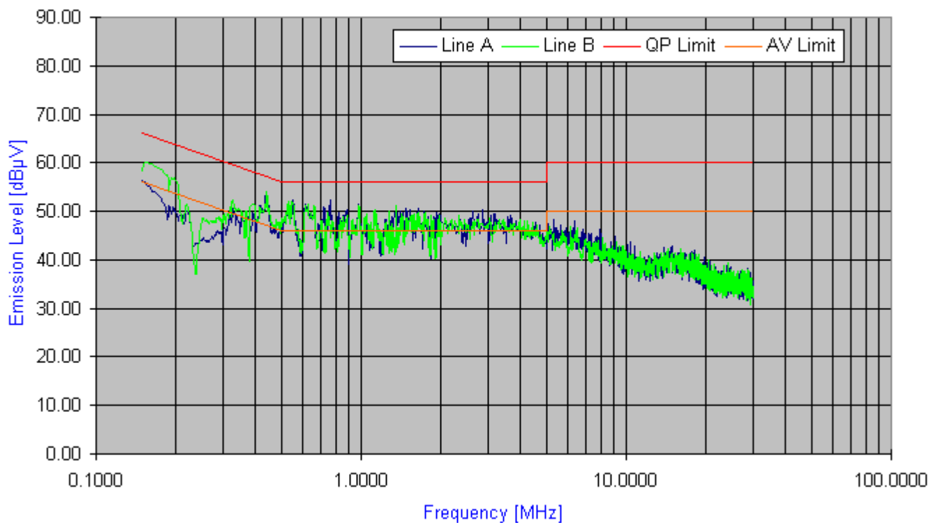
Plot 7-1. Line-Conducted Test Plot
