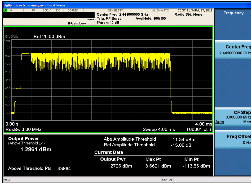
Plot 6-26. Average Conducted Power (3Mbps – Ch. 39)
