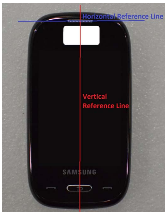
SAR Test Setup Photo 6 – DUT Horizontal and Vertical Reference Lines
