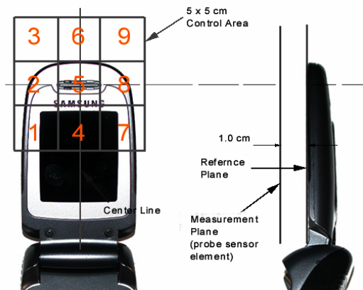
Figure 13 E/H-Field Emissions Test Setup Diagram
