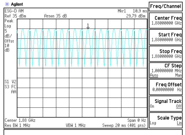
Figure 25 80% AM Signal
