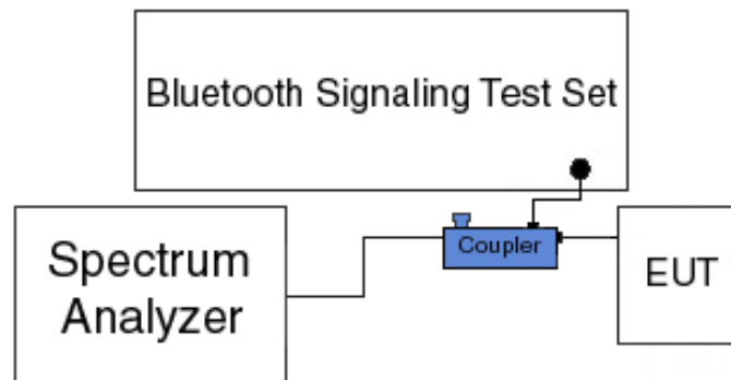
Figure 6-2. Test Instrument & Measurement Setup
