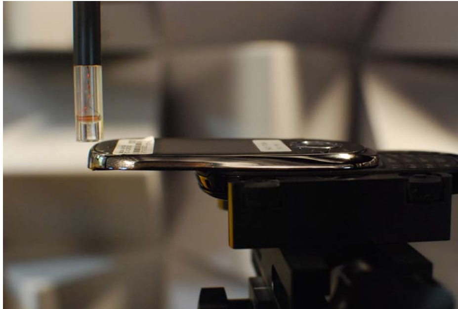
Figure 12-1 Test Setup for Wireless Device
